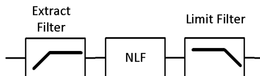
Figure 13. Treble Enhancement
