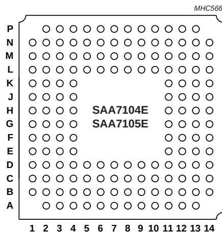
Fig.2 Pin configuration.
