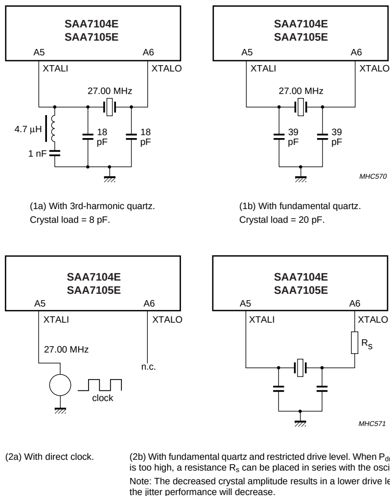
Fig.17 Oscillator application.
