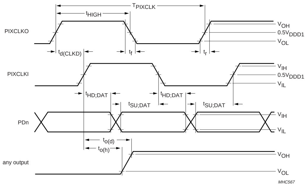
Fig.11 Input/output timing specification.
