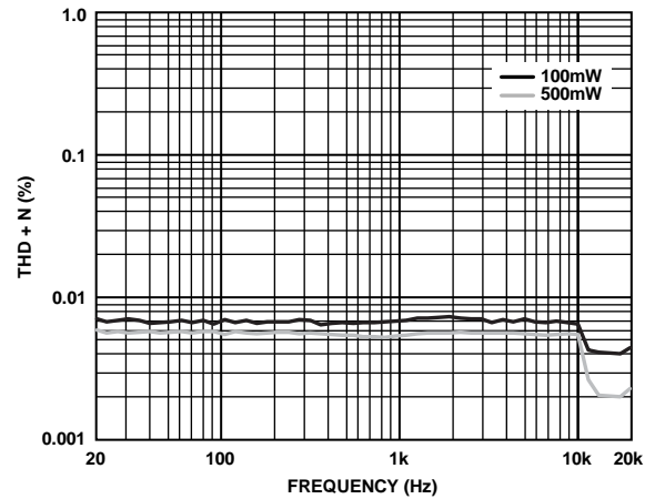
Figure 17. THD + N vs. Frequency into R_L = 8 \Omega , PV_{DD} = 4.5 V
