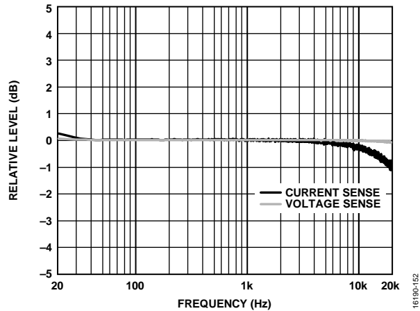
Figure 57. Current Voltage (I/V) Sense Frequency Response, -20 dBFS Input Signal, PV_{DD} = 12 V , Analog Gain = 12.6
