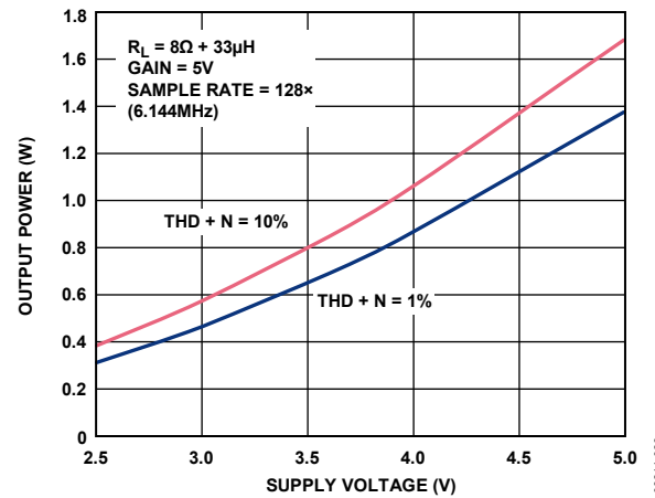
Figure 21. Maximum Output Power vs. Supply Voltage, Gain = 5 V, R_L = 8\Omega , f_s = 128\times
