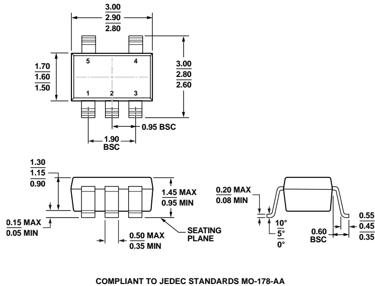
Figure 40. 5-Lead Small Outline Transistor Package [SOT-23] (RJ-5) Dimensions shown in millimeters
