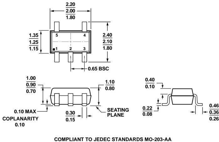
Figure 41. 5-Lead Thin Shrink Small Outline Transistor Package [SC70] (KS-5) Dimensions shown in millimeters
