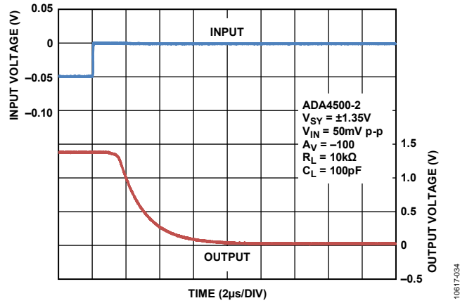
Figure 41. Positive Overload Recovery, V_{SY} = \pm 1.35V
