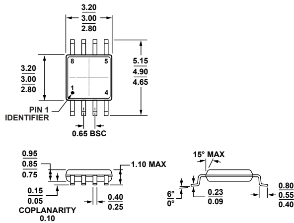
COMPLIANT TO JEDEC STANDARDS MO-187-AA Figure 68. 8-Lead Mini Small Outline Package [MSOP] (RM-8) Dimensions shown in millimeters
