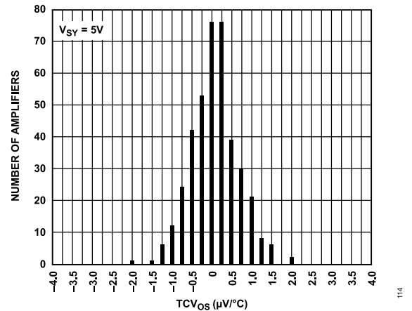
Figure 14. Input Offset Voltage Drift ( TCV_{OS} ) Distribution ( -40^\circ\text{C} to +125^\circ\text{C} ), V_{SY} = 5\text{V}
