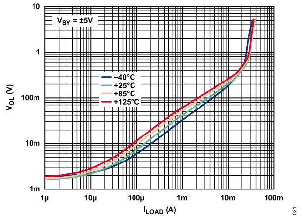
Figure 25. Output Voltage Low ( V_{OL} ) to Supply Rail vs. Load Current ( I_{LOAD} ) over Temperature, V_{SY} = \pm 5 V
