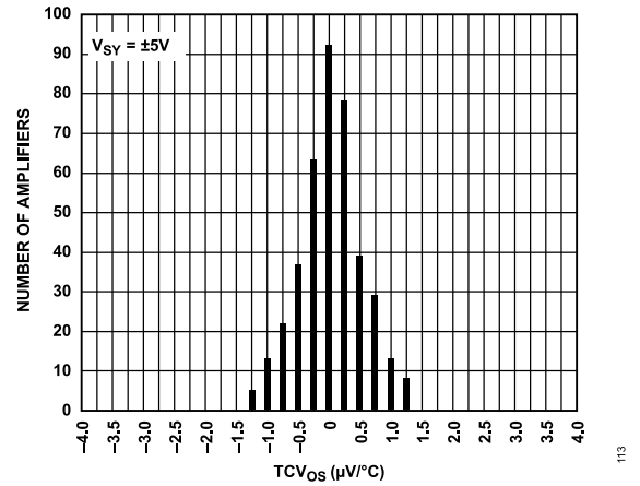
Figure 13. Input Offset Voltage Drift ( TCV_{OS} ) Distribution ( -40^\circ\text{C} to +125^\circ\text{C} ), V_{SY} = \pm 5\text{V}
