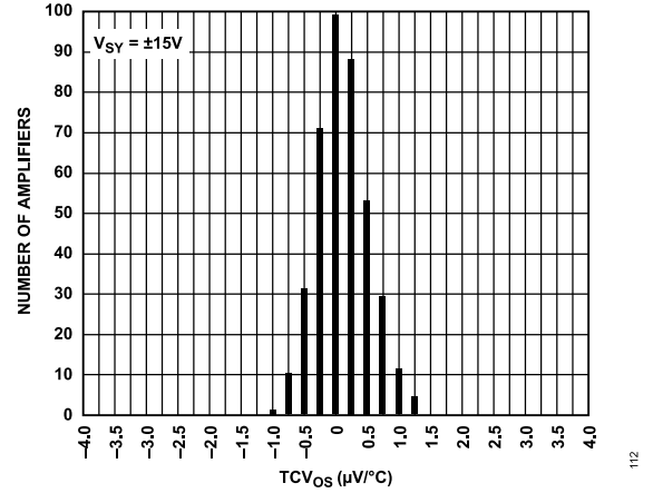
Figure 12. Input Offset Voltage Drift ( TCV_{OS} ) Distribution ( -40^\circ\text{C} to +125^\circ\text{C} ), V_{SY} = \pm 15\text{V}
