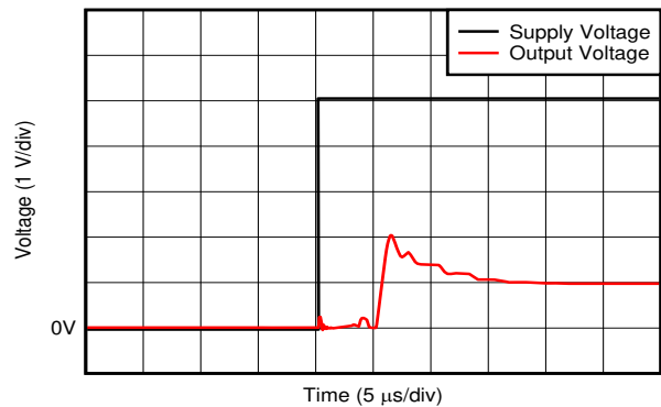
Figure 6-42. Start-Up Response
