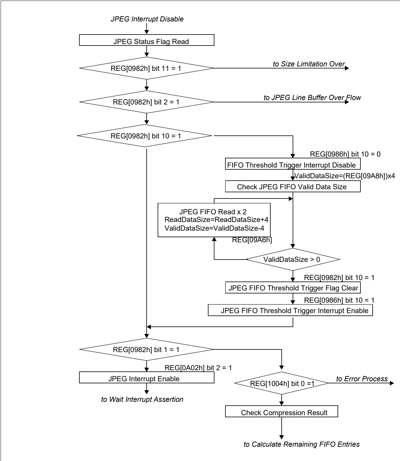
Figure 19-4: JPEG Encoding Process (3 of 4)
