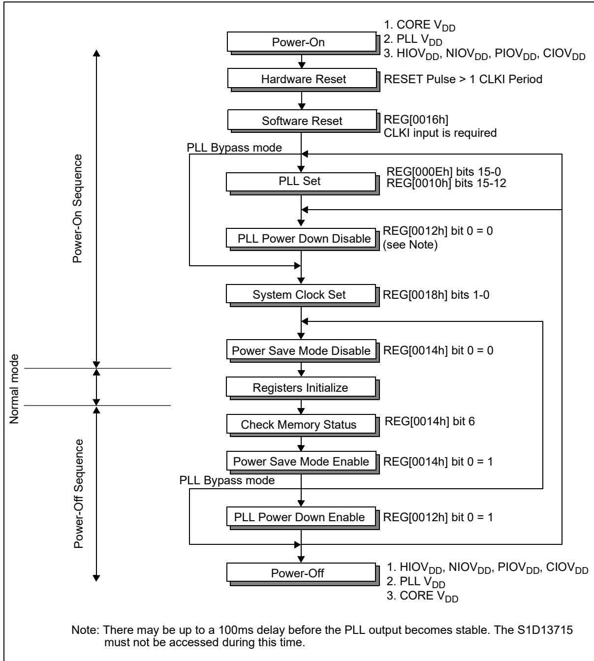
Figure 11-1: Power-On/Power-Off Sequence
