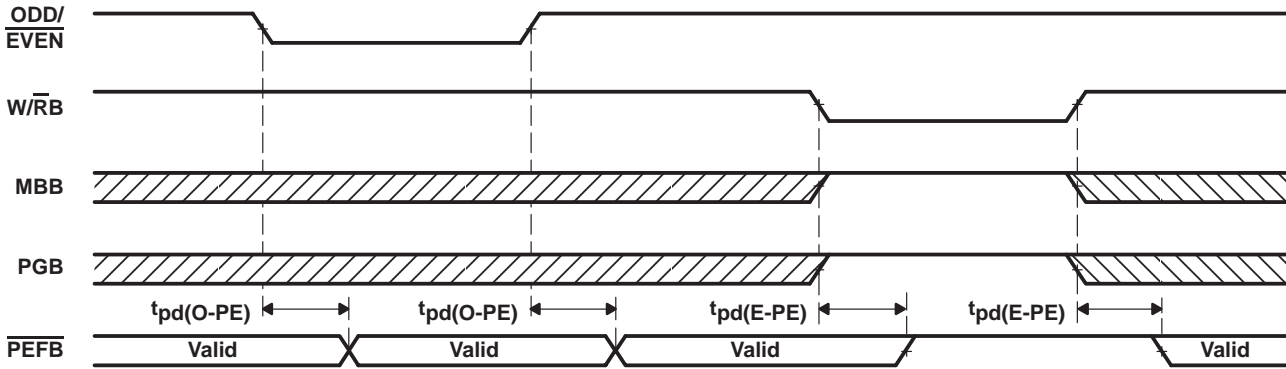
Figure 17. ODD/ \overline{\text{EVEN}} , \text{W}/\overline{\text{RB}} , \text{MBB} , and \text{PGB} to \overline{\text{PEFB}} Timing
