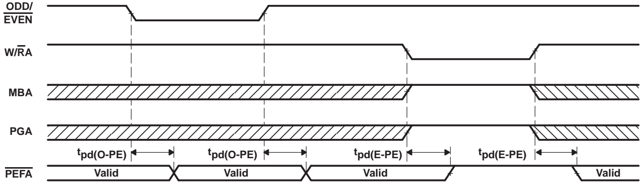
Figure 16. ODD/ \overline{\text{EVEN}} , \text{W}/\overline{\text{RA}} , \text{MBA} , and \text{PGA} to \overline{\text{PEFA}} Timing
