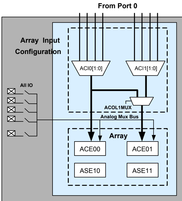
Figure 2. Analog System Block Diagram
