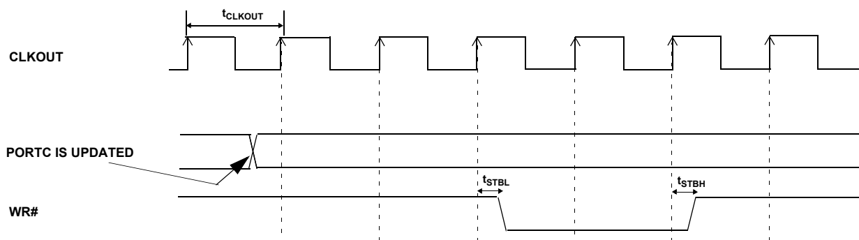
Figure 16. WR# Strobe Function when PORTC is Accessed by 8051
