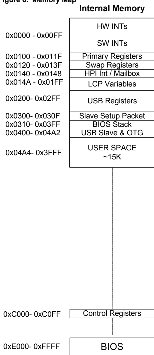
Figure 6. Memory Map
