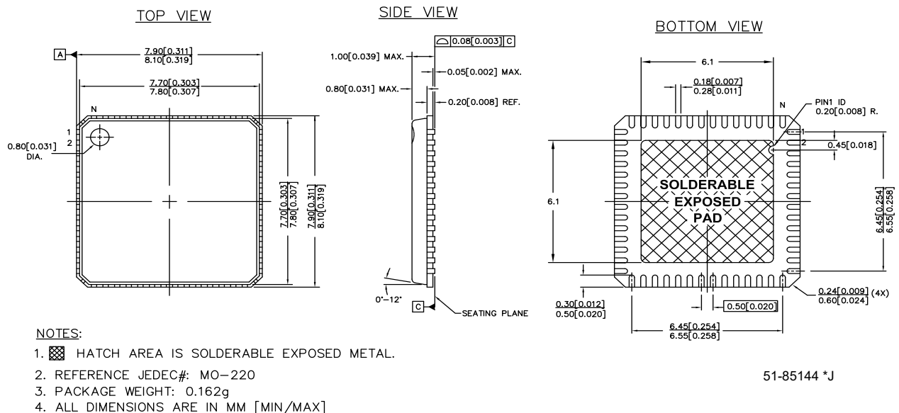
Figure 7. 56-pin QFN 8 \times 8 mm LF56A (Subcon Punch Type with 6.1 \times 6.1 EPad)
