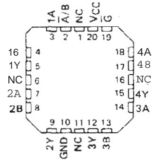
SN54IS157, SN54S157, SN54IS158, SN54S158 ... FK PACKAGE (TOP VIEW)
