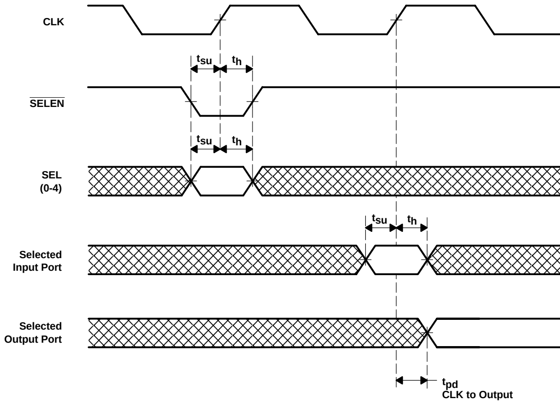
timing diagram
