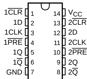
D, DGV, OR PW PACKAGE (TOP VIEW)
