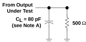
LOAD CIRCUIT
