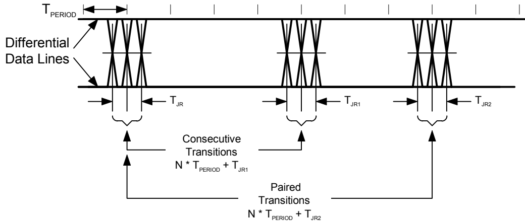
Figure 24-3. Receiver Jitter Tolerance
