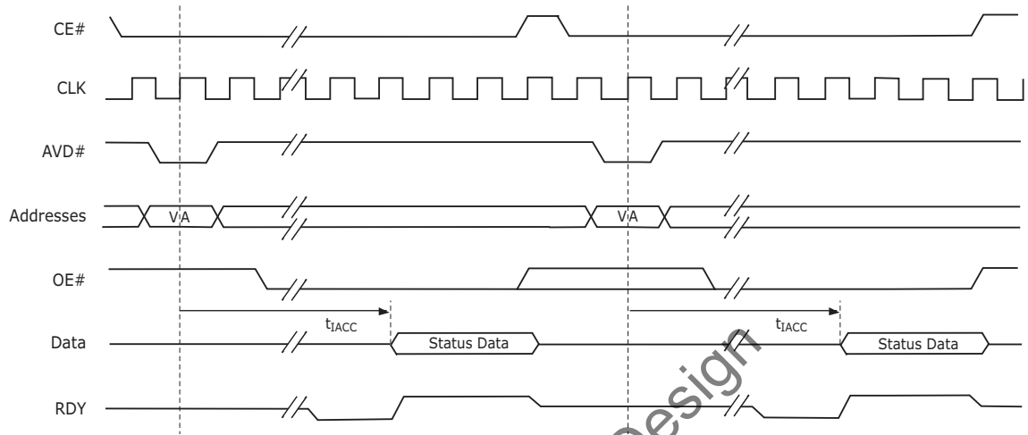
Figure 11.20 Synchronous Data Polling Timings/Toggle Bit Timings
