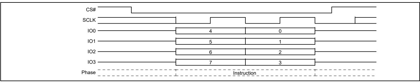
Figure 89 Program or Erase Suspend command sequence QPI mode
