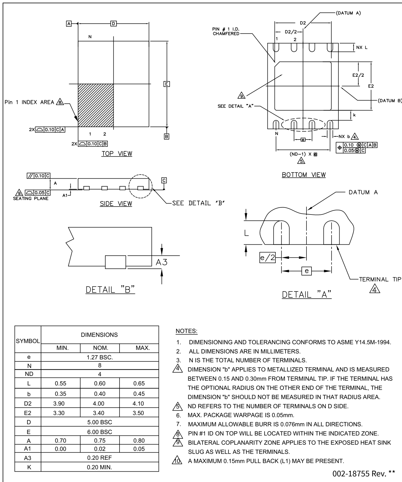
Figure 153 8-lead DFN ((5.0 × 6.0 × 0.8 mm) WND008, 4.0 × 3.4 mm E-Pad (Sawn)) package outline, 002-18755
