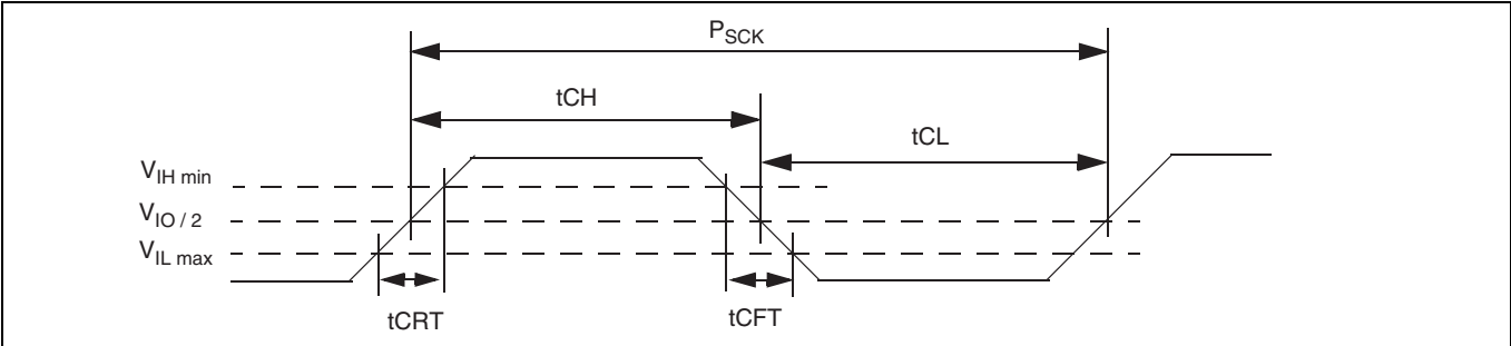
Figure 34 Clock timing
