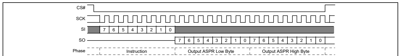
Figure 90 ASPRD command
