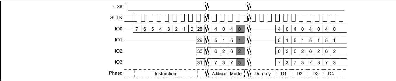
Figure 12 Quad I/O command
