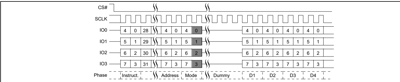
Figure 13 Quad I/O Read command in QPI mode
