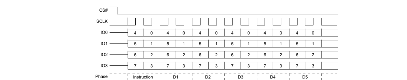
Figure 44 Read Identification (RDID) QPI mode command
