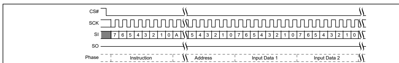
Figure 75 Page Program (PP 02h or 4PP 12h) command sequence [51]
