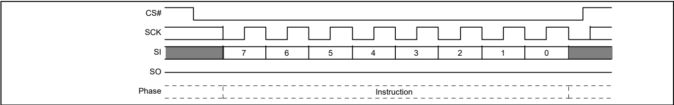
Figure 52 Clear Status Register (CLSR) command sequence
