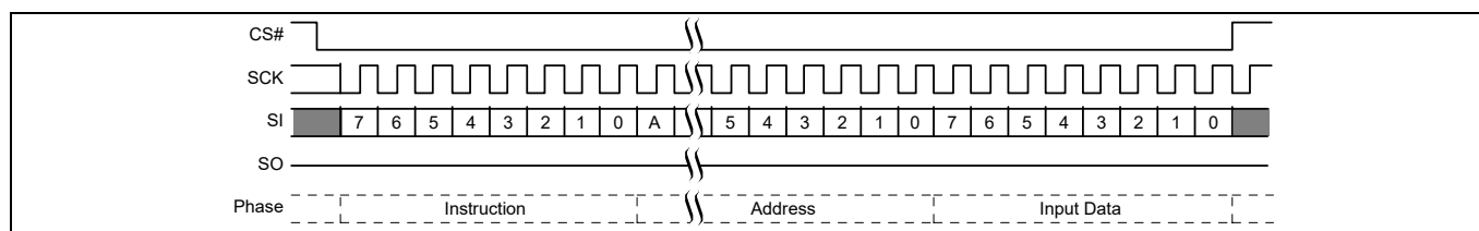
Figure 93 DYBWR command sequence [59, 60]
