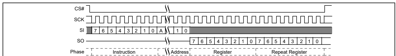
Figure 91 DYBRD command sequence [57, 58]
