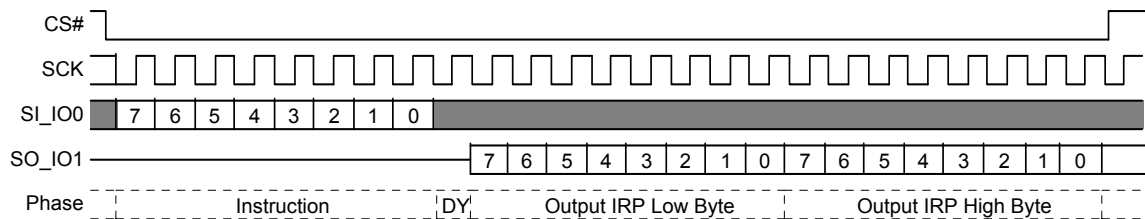
Figure 9.81 IRPRD Command Sequence
