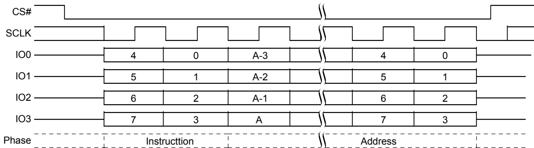
Figure 9.57 Half Block Erase (HBE 52h or 4HBE 53h) QPI Mode Command Sequence
