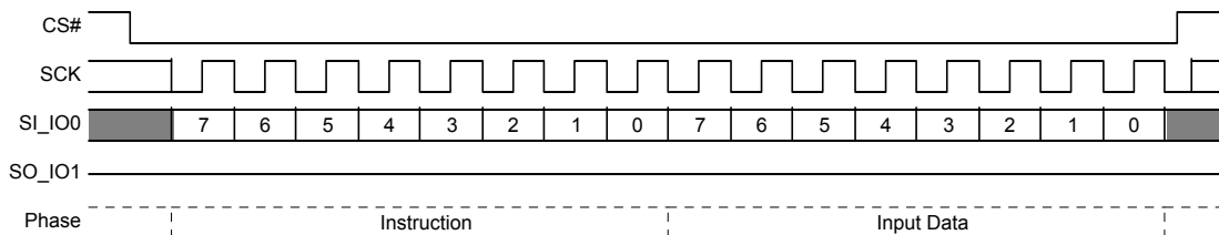
Figure 9.23 Program DLRNV (PDLRNV) Command Sequence
