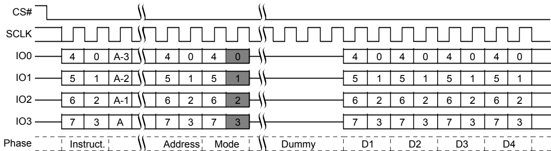
Figure 9.46 Quad I/O Read Initial Access Command Sequence QPI mode
