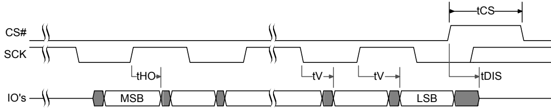
Figure 5.16 SPI DDR Output Timing
