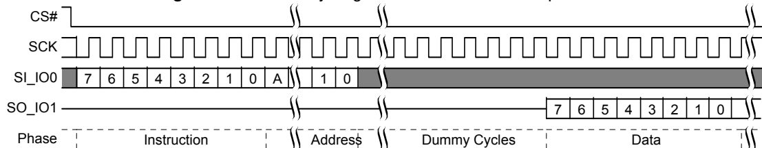
Figure 9.33 Read Any Register Read Command Sequence
