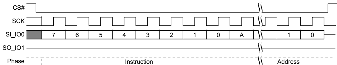
Figure 9.58 Block Erase (BE D8h or 4BE DCh) Command Sequence
