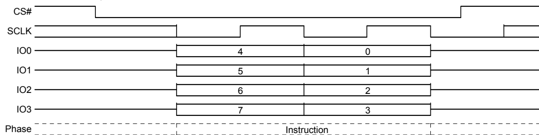
Figure 9.76 Global IBL Lock (GBL) Command Sequence QPI mode
