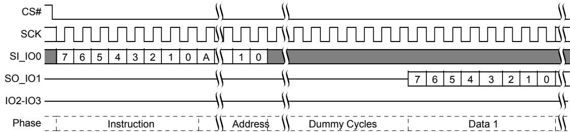
Figure 9.40 Fast Read (FAST_READ) Command Sequence
