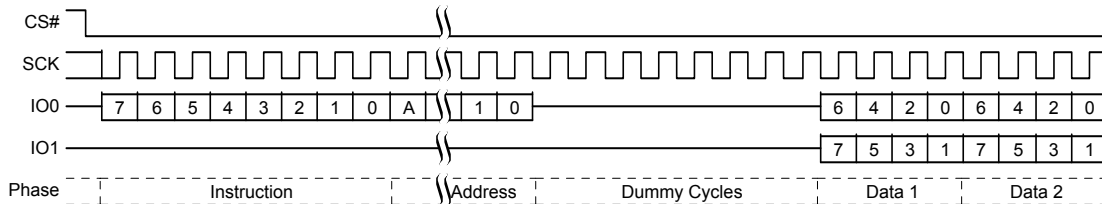
Figure 9.41 Dual Output Read Command Sequence
