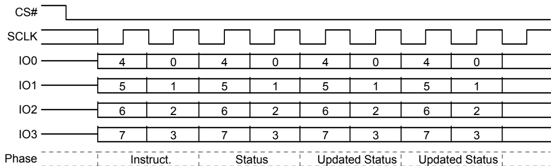
Figure 9.10 Read Status Register-1 (RDSR1) QPI Mode Command
