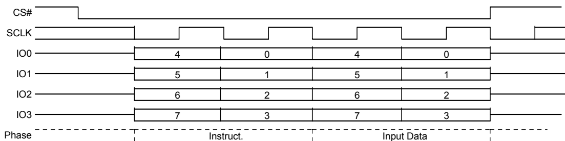
Figure 9.26 Write DLRV (WDLRV) Command Sequence – QPI Mode
