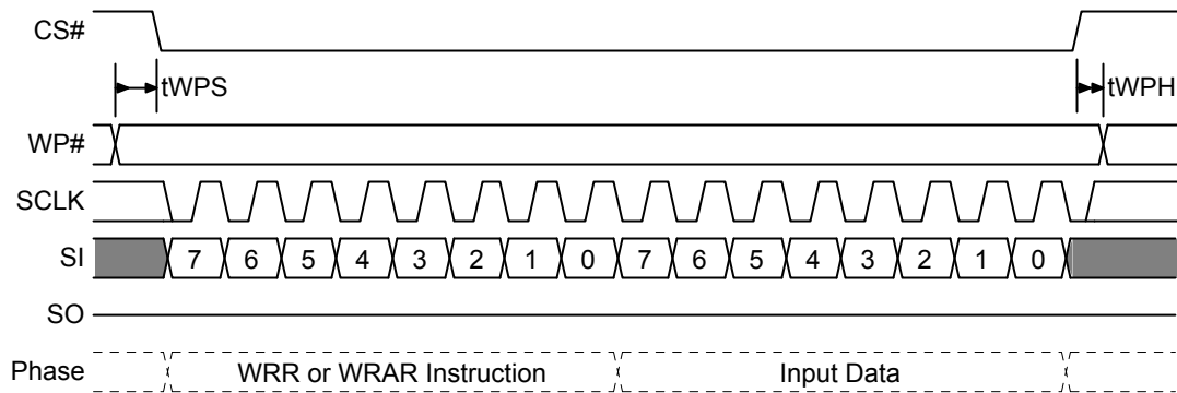
Figure 5.14 WP# Input Timing
