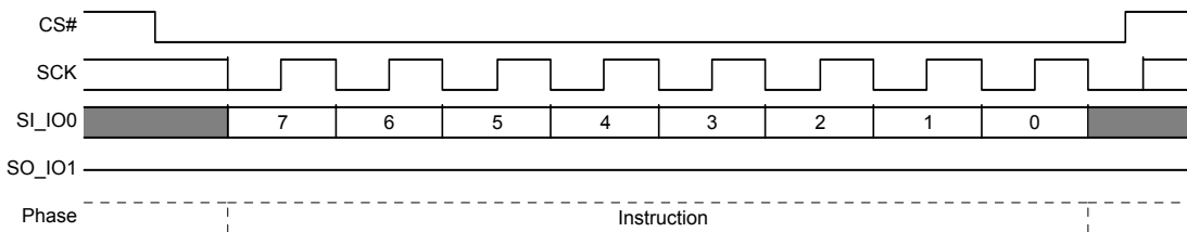
Figure 9.19 Write Enable for Volatile Registers (WRENV) Command Sequence
