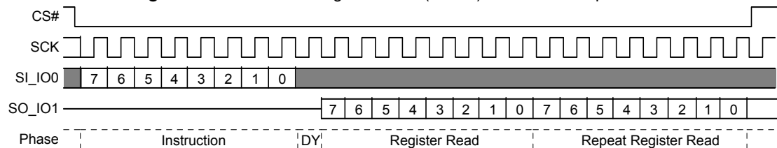
Figure 9.85 Protection Register Read (PRRD) Command Sequence
