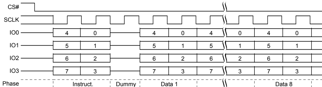
Figure 9.90 Password Read (PASSRD) Command Sequence – QPI Mode
