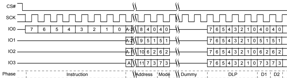
Figure 9.48 DDR Quad I/O Read Initial Access
