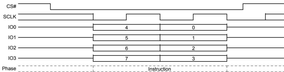
Figure 9.63 Program or Erase Suspend Command Sequence QPI mode
