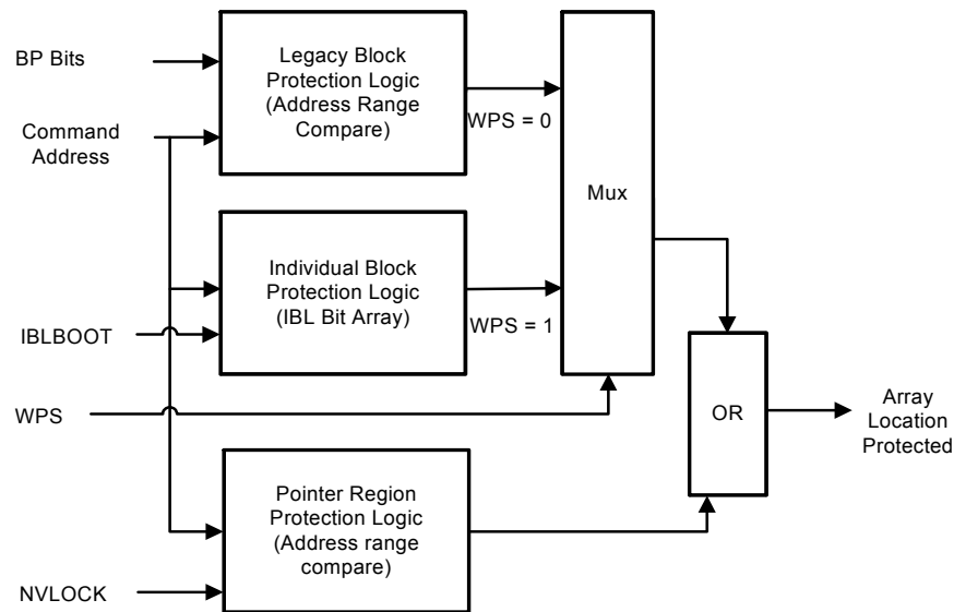
Figure 8.1 WPS Selection of LBP or IBL and PRP Array Protection
