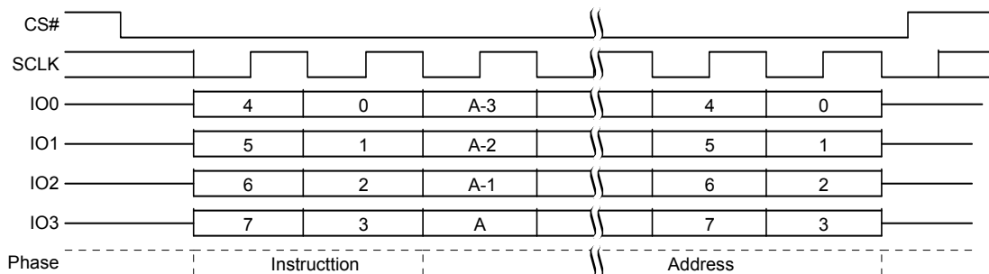
Figure 9.74 IBUL Command Sequence QPI Mode
