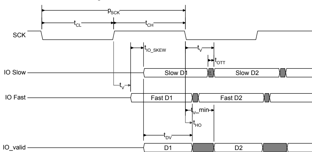
Figure 5.17 SPI DDR Data Valid Window
