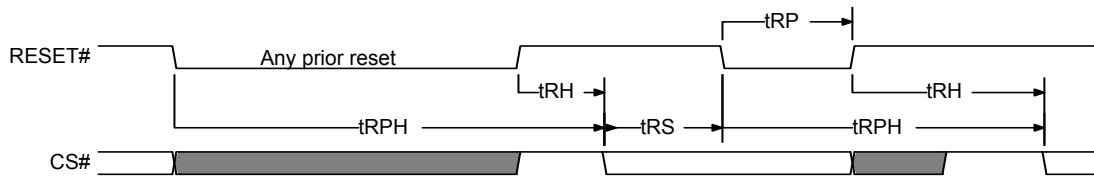
Figure 5.7 Hardware Reset using RESET# Input
