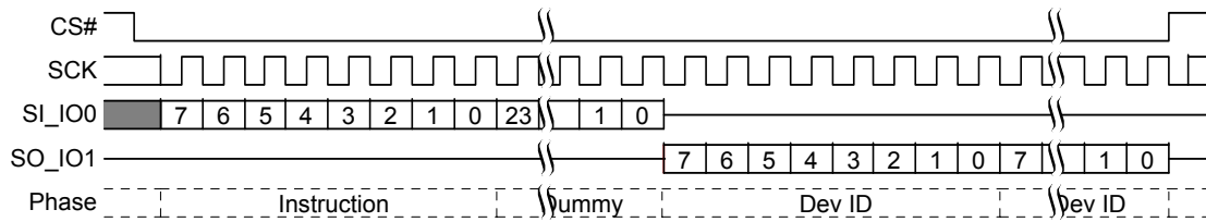
Figure 9.101 Read Identification (RES) Command Sequence
