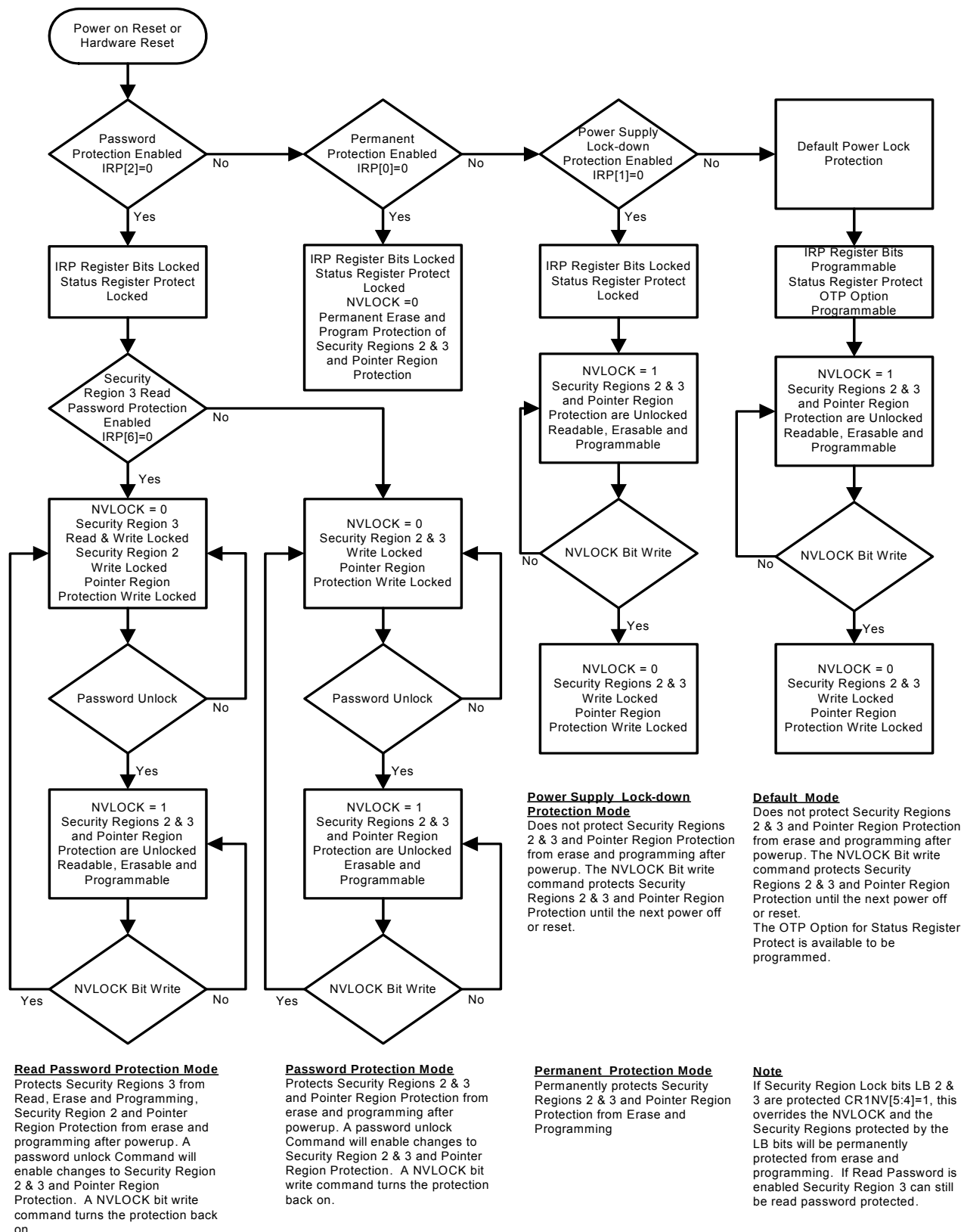
Figure 8.3 Permanent, Password and Power Supply Lock-down Protection Overview
