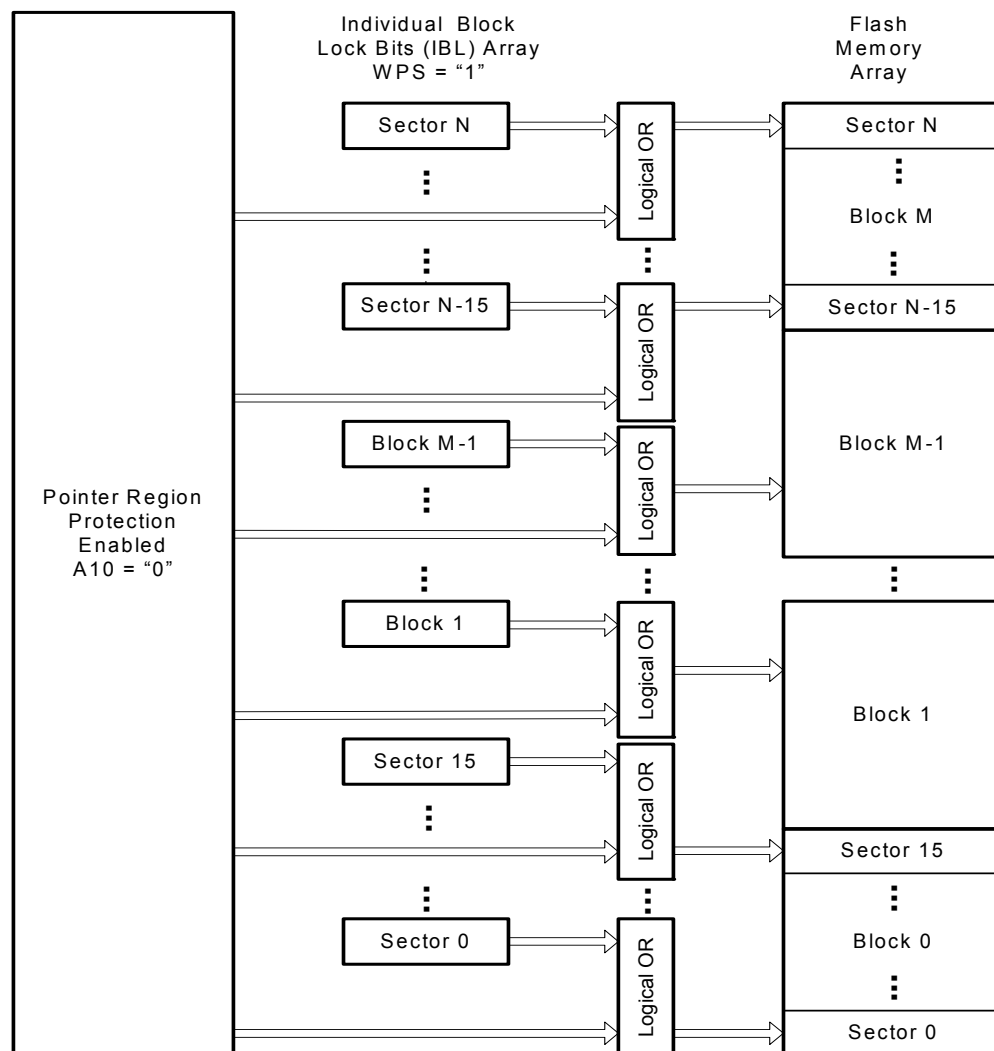
Figure 8.2 Individual Block Lock / Pointer Region Protection Control
