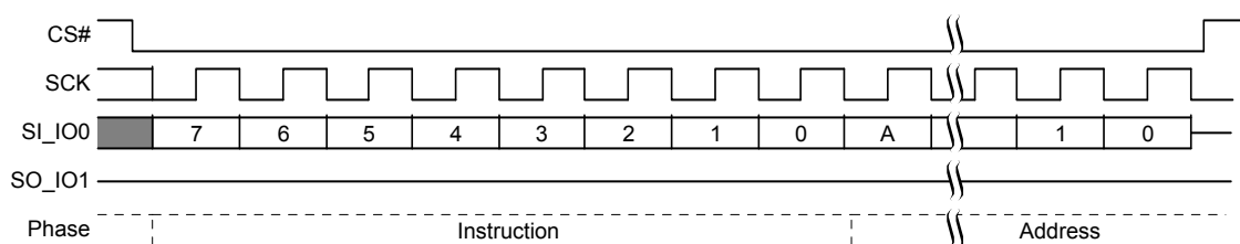
Figure 9.56 Half Block Erase (HBE 52h or 4HBE 53h) Command Sequence
