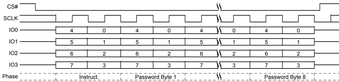
Figure 9.94 Password Unlock (PASSU) Command Sequence QPI mode
