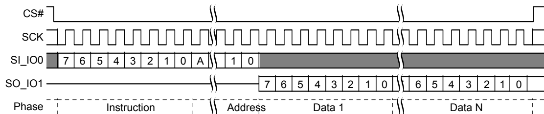
Figure 9.39 Read Command Sequence
