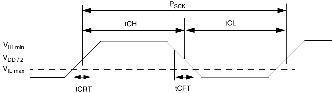
Figure 5.10 Clock Timing
