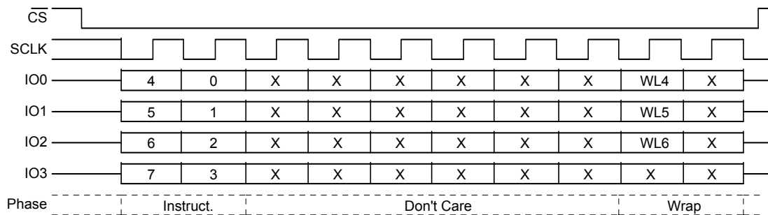
Figure 9.36 Set Burst Length Command Sequence QPI Mode
