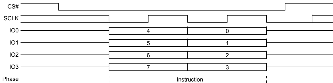
Figure 9.22 Clear Status Register (CLSR) QPI Mode
