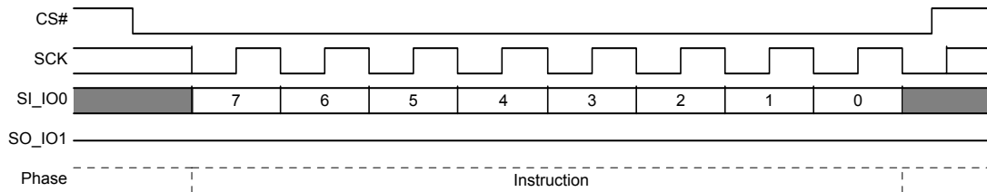
Figure 9.15 Write Enable (WREN) Command Sequence
