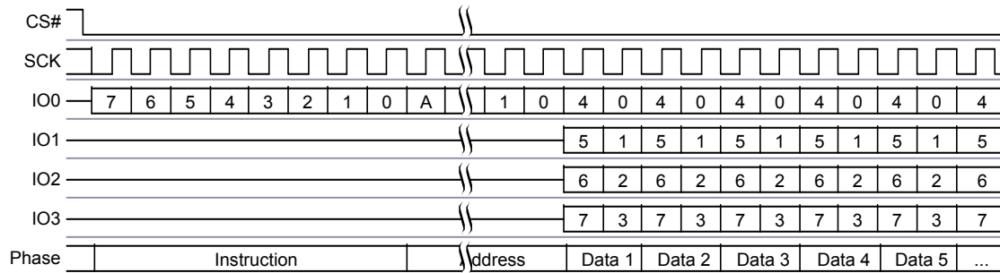
Figure 9.53 Quad Page Program Command Sequence
