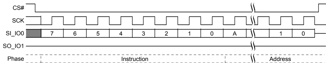
Figure 9.71 IBL Command Sequence
