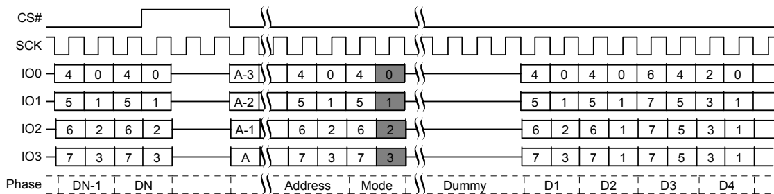
Figure 9.47 Continuous Quad I/O Read Command Sequence
