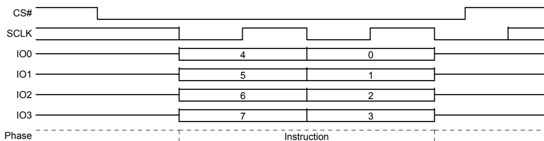
Figure 9.66 Erase or Program Resume command Sequence QPI mode
