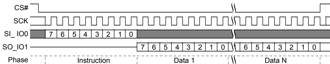
Figure 9.1 Read Identification (RDID) Command Sequence
