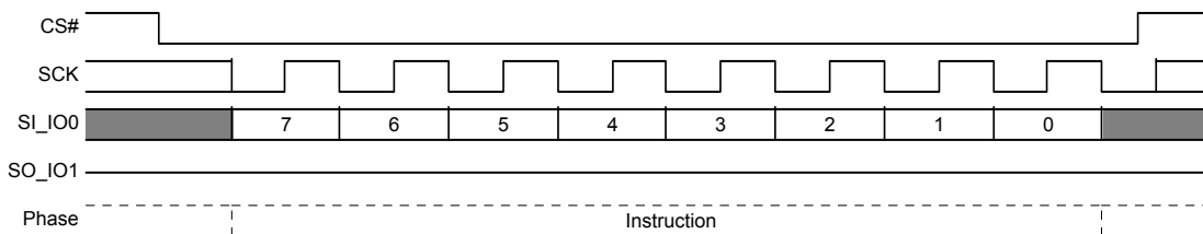
Figure 9.37 Enter QPI Mode (QPIEN 38h) Command Sequence
