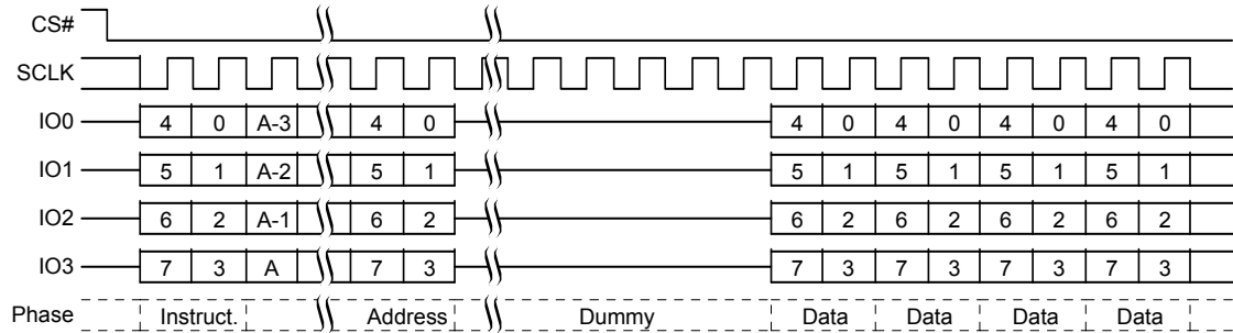
Figure 9.34 Read Any Register, QPI Mode, Command Sequence
