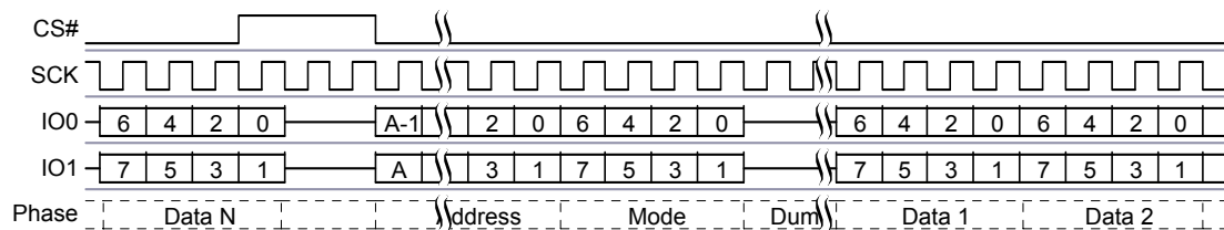
Figure 9.44 Dual I/O Continuous Read Command Sequence
