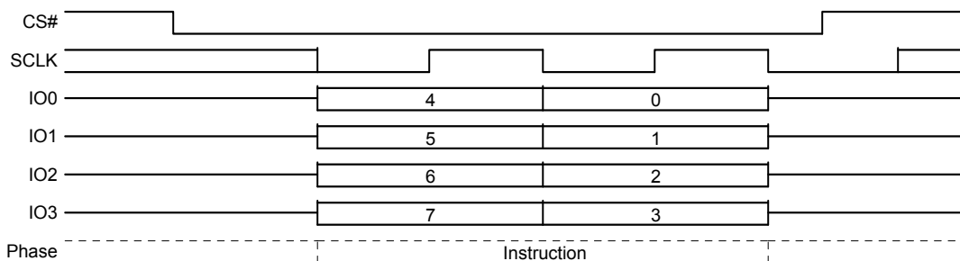
Figure 9.96 Software Reset / Mode Bit Command Sequence – QPI Mode
