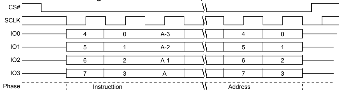
Figure 9.80 SPRP Command Sequence QPI Mode
