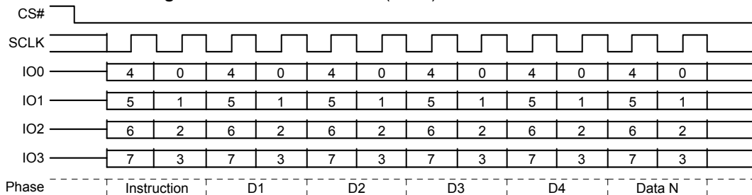
Figure 9.2 Read Identification (RDID) QPI Mode Command
