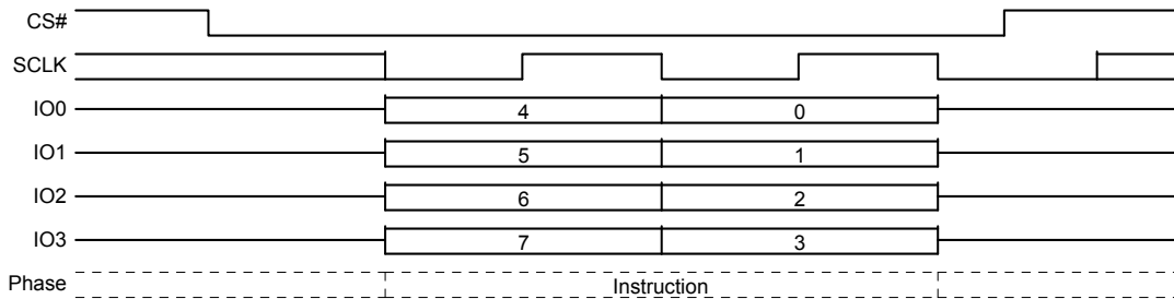
Figure 9.38 Exit QPI (QPIEX F5h) Command Sequence
