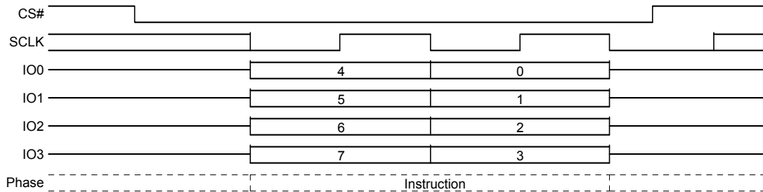
Figure 9.18 Write Disable (WRDI) Command Sequence QPI Mode
