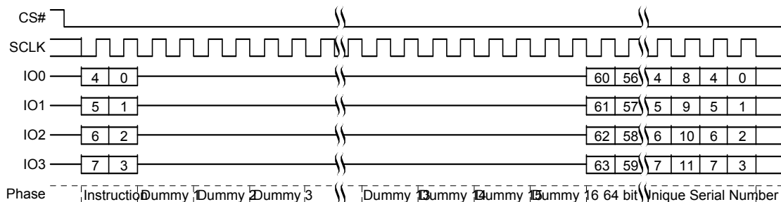
Figure 9.8 Read Unique ID (RUID) QPI Mode Command
