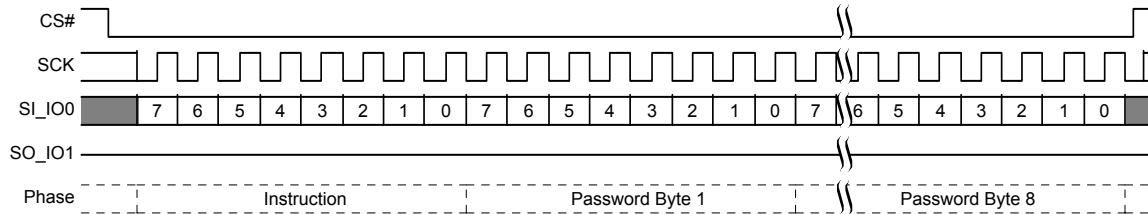
Figure 9.91 Password Program (PASSP) Command Sequence
