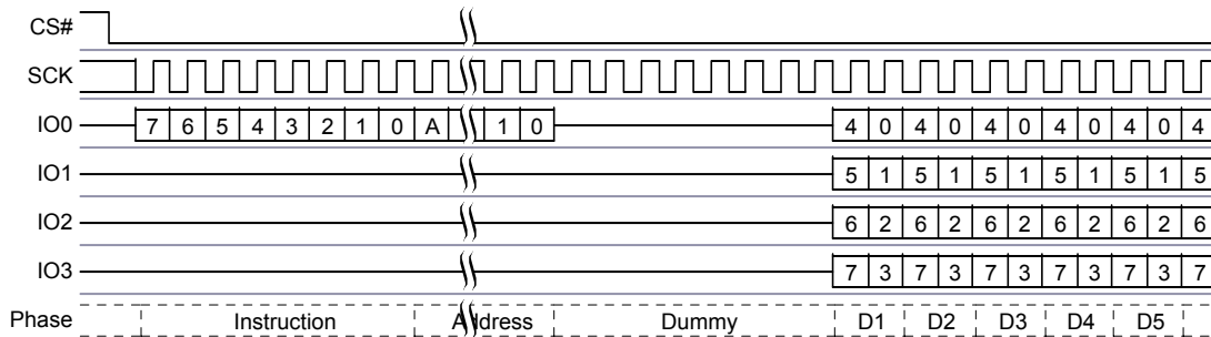
Figure 9.42 Quad Output Read Command Sequence
