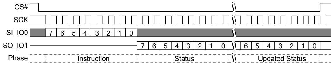
Figure 9.9 Read Status Register-1 (RDSR1) Command Sequence
