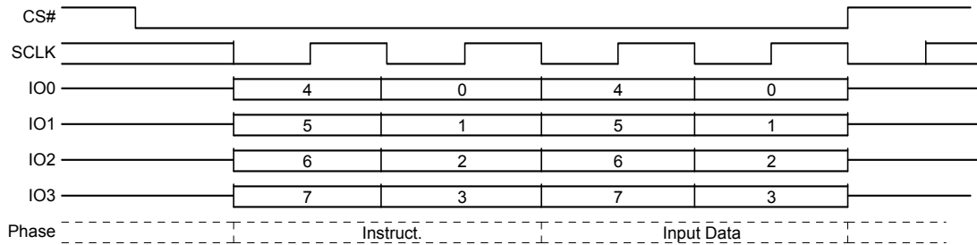
Figure 9.24 Program DLRNV (PDLRNV) Command Sequence – QPI Mode
