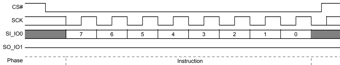
Figure 9.31 Exit 4 Byte Address Mode (4BEX E9h) Command Sequence
