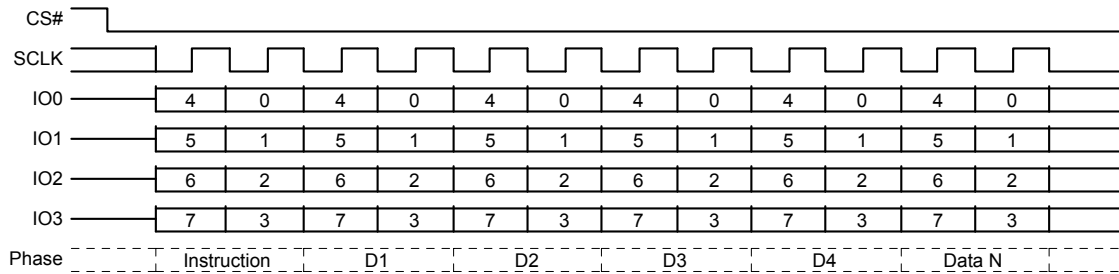
Figure 9.3 Read Quad Identification (RDQID) Command Sequence QPI Mode
