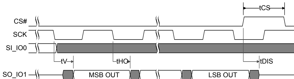
Figure 5.12 SPI Single Bit Output Timing
