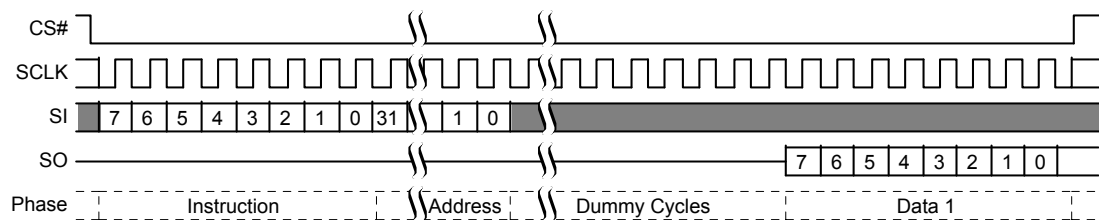
Figure 3.6 Single Bit Wide I/O Command with latency
