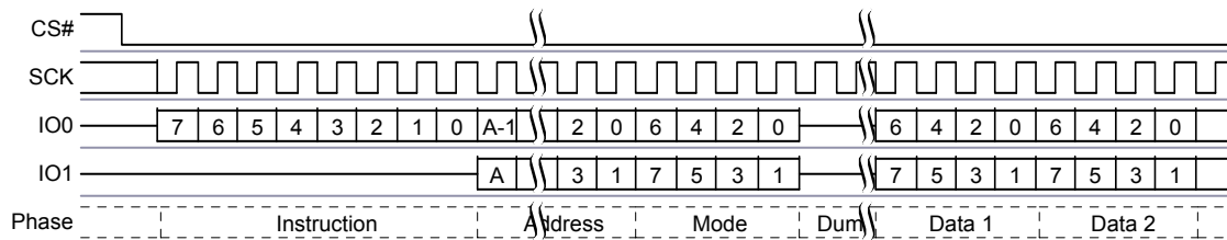
Figure 9.43 Dual I/O Read Command Sequence
