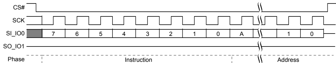
Figure 9.54 Sector Erase (SE 20h or 4SE 21h) Command Sequence
