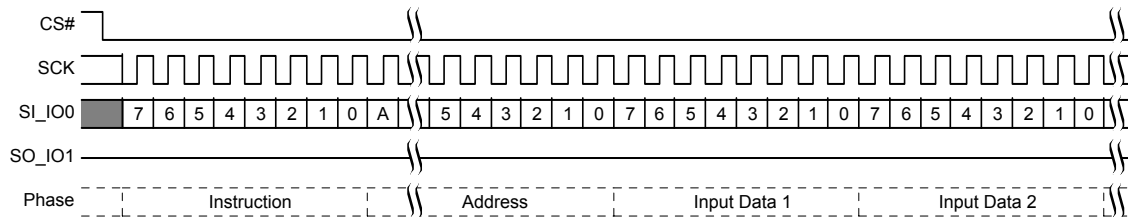
Figure 9.51 Page Program (PP 02h or 4PP 12h) Command Sequence
