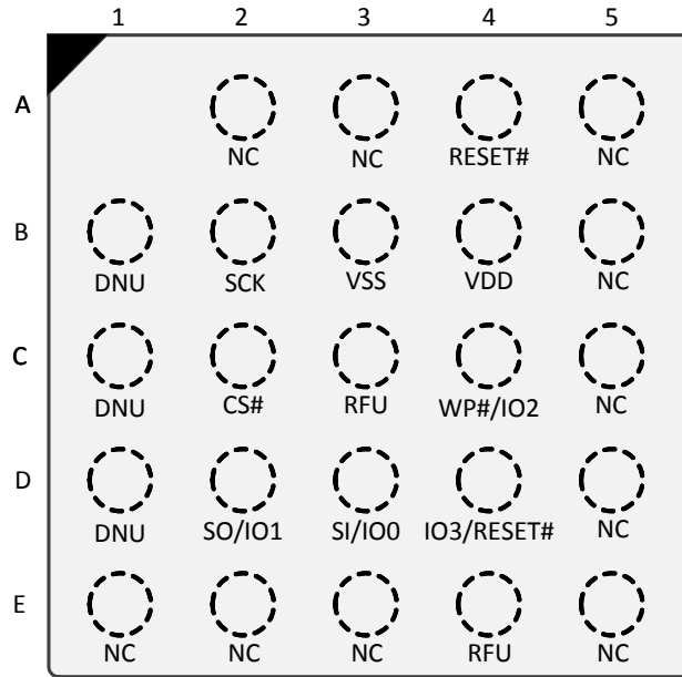
Figure 6.3 24-Ball BGA, 5x5 Ball Footprint (FAB024), Top View
