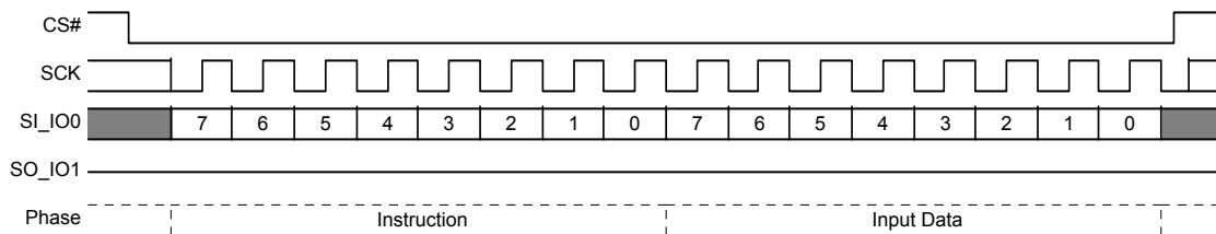
Figure 9.25 Write DLRV (WDLRV) Command Sequence
