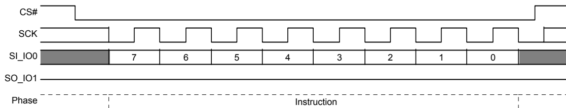
Figure 9.87 Protection Register Lock (PRL) Command Sequence
