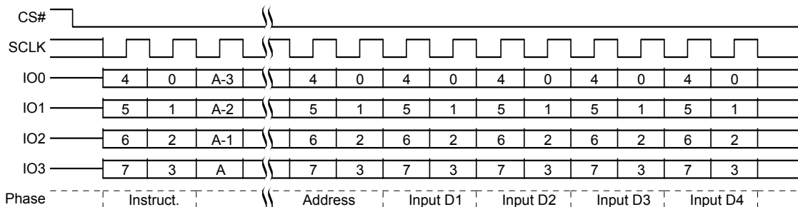
Figure 9.52 Page Program (PP 02h or 4PP 12h) QPI Mode Command Sequence
