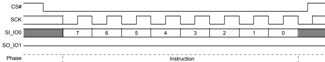
Figure 9.60 Chip Erase Command Sequence
