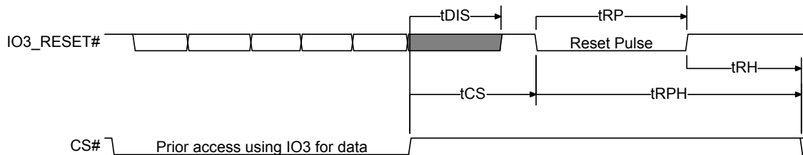
Figure 5.9 Hardware Reset when Quad or QPI Mode and IO3 / RESET# are Enabled
