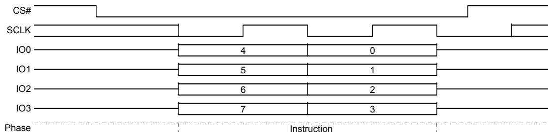
Figure 9.78 Global IBL Unlock (GBUL) Command Sequence QPI mode
