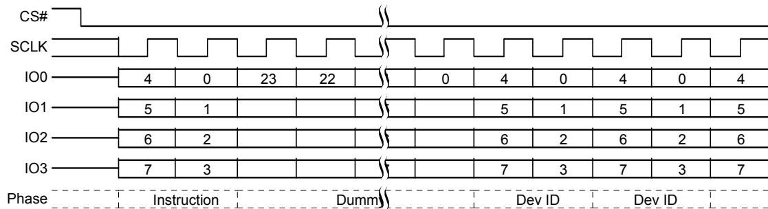
Figure 9.102 Read Identification (RES) QPI Mode Command
