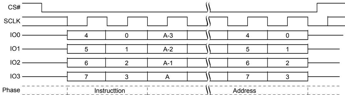
Figure 9.59 Block Erase (BE D8h or 4BE DCh) QPI Mode Command Sequence
