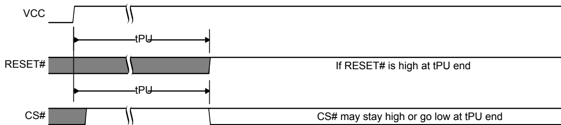
Figure 5.5 Reset high at the end of POR
