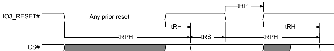
Figure 5.8 Hardware Reset when Quad or QPI Mode is not enabled and IO3 / RESET# is Enabled
