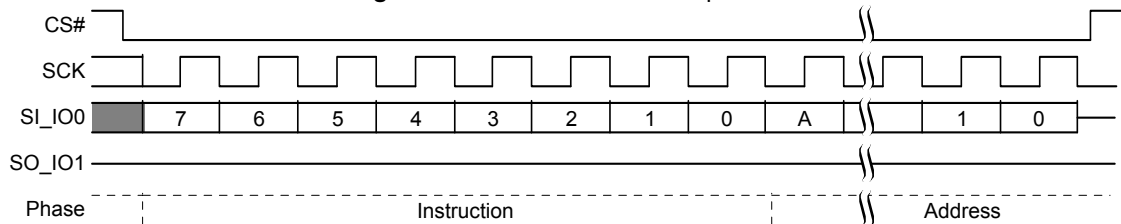
Figure 9.73 IBUL Command Sequence
