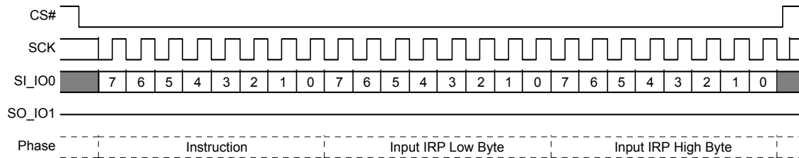
Figure 9.83 IRP Program (IRPP) Command
