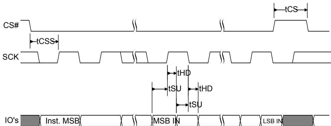
Figure 5.15 SPI DDR Input Timing
