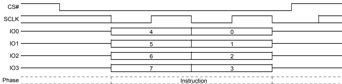
Figure 9.16 Write Enable (WREN) Command Sequence QPI Mode
