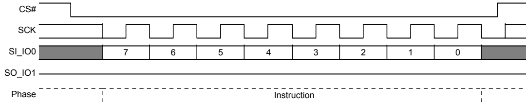
Figure 9.21 Clear Status Register (CLSR) Command Sequence
