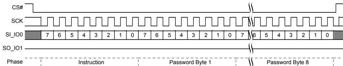
Figure 9.93 Password Unlock (PASSU) Command Sequence
