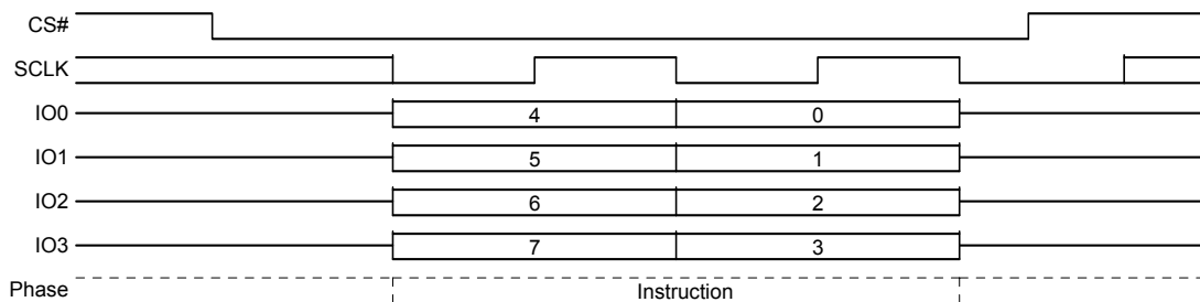
Figure 9.32 Exit 4 Byte Address QPI Mode
