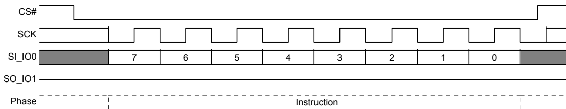
Figure 9.77 Global IBL Unlock (GBUL) Command Sequence
