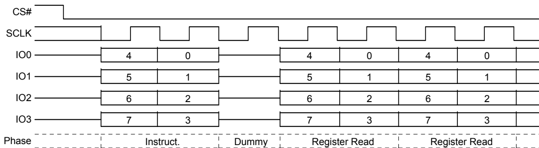
Figure 9.28 DLP Read (DLPRD) Command Sequence – QPI Mode
