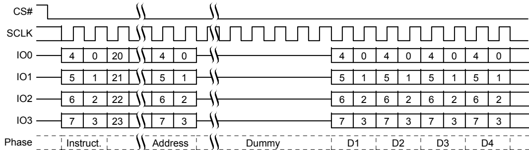
Figure 9.6 RSFDP QPI Mode Command Sequence
