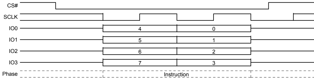
Figure 9.98 Deep Power Down (DPD) Command Sequence – QPI Mode
