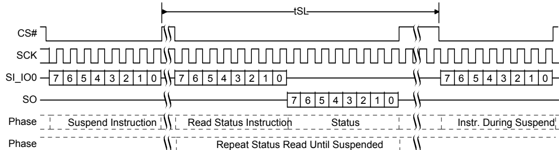
Figure 9.64 Program or Erase Suspend Command with Continuing Instruction Commands Sequence
