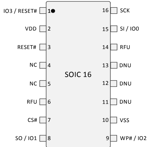
Figure 6.1 16-Lead SOIC Package (SO3016), Top View
