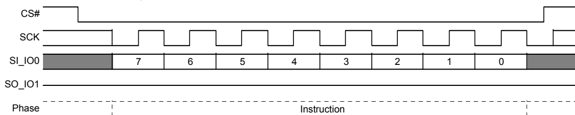
Figure 9.97 Deep Power Down (DPD) Command Sequence
