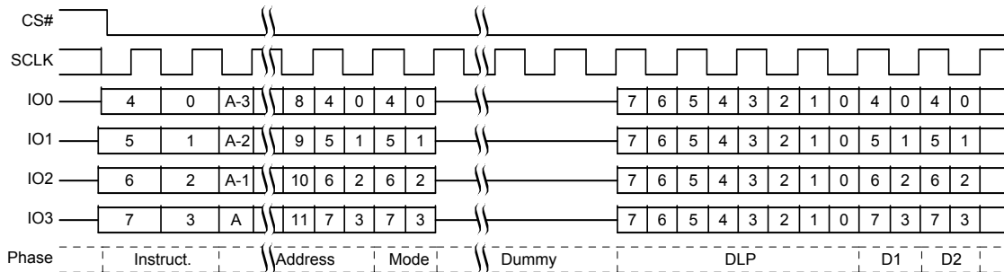
Figure 9.49 DDR Quad I/O Read Initial Access QPI Mode
