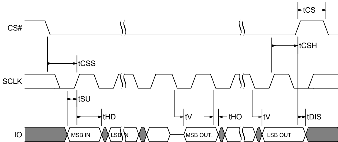
Figure 5.13 SDR MIO Timing
