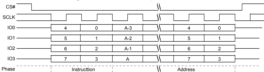
Figure 9.72 IBL Command Sequence QPI Mode
