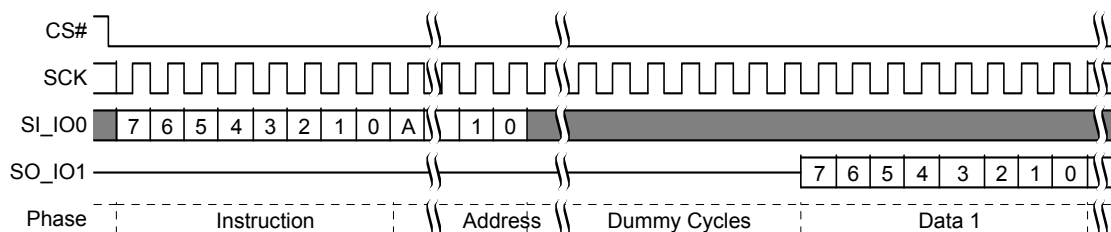
Figure 9.67 Security Regions Read Command Sequence
