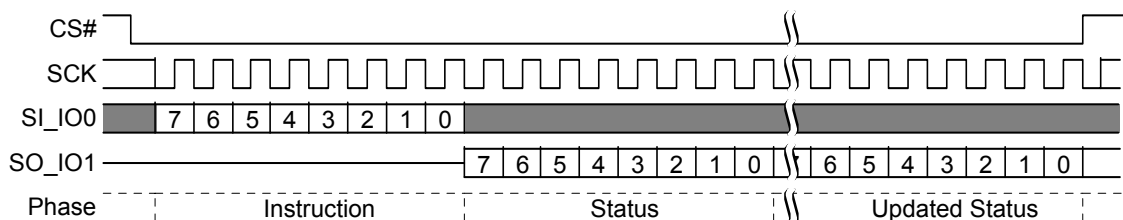
Figure 9.11 Read Status Register-2 (RDSR2) Command
