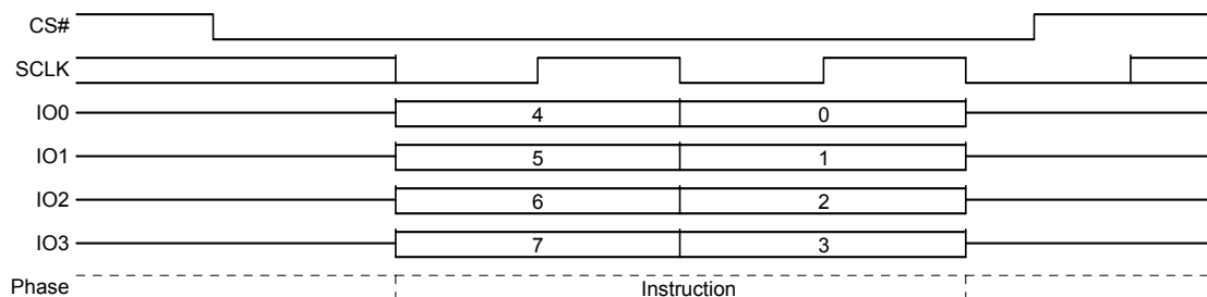
Figure 9.88 Protection Register Lock (PRL) Command Sequence – QPI Mode
