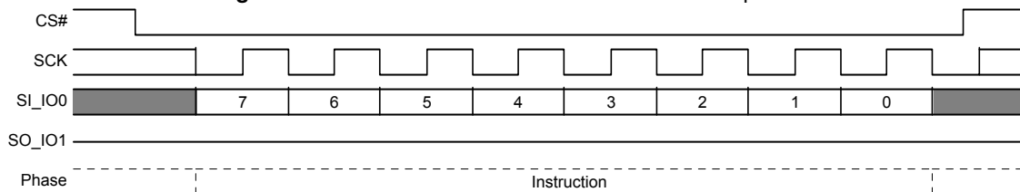
Figure 9.95 Software / Mode Bit Reset Command Sequence
