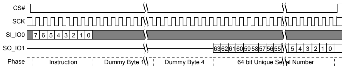
Figure 9.7 Read Unique ID (RUID) Command Sequence
