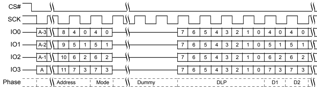
Figure 9.50 Continuous DDR Quad I/O Read Subsequent Access
