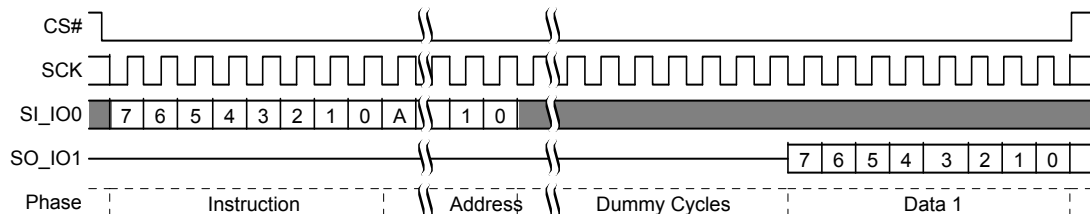
Figure 9.5 RSFDP Command Sequence
