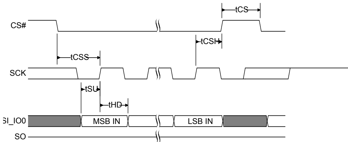
Figure 5.11 SPI Single Bit Input Timing
