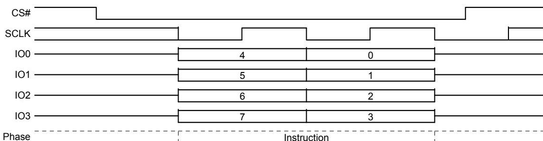
Figure 9.61 Chip Erase Command Sequence QPI Mode
