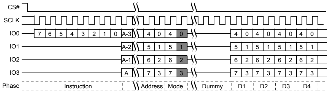
Figure 9.45 Quad I/O Read Initial Access Command Sequence
