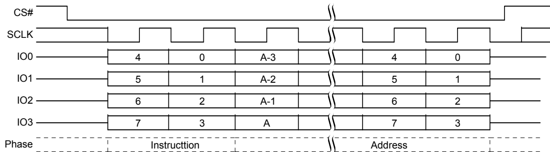
Figure 9.55 Sector Erase (SE 20h or 4SE 21h) QPI Mode Command Sequence
