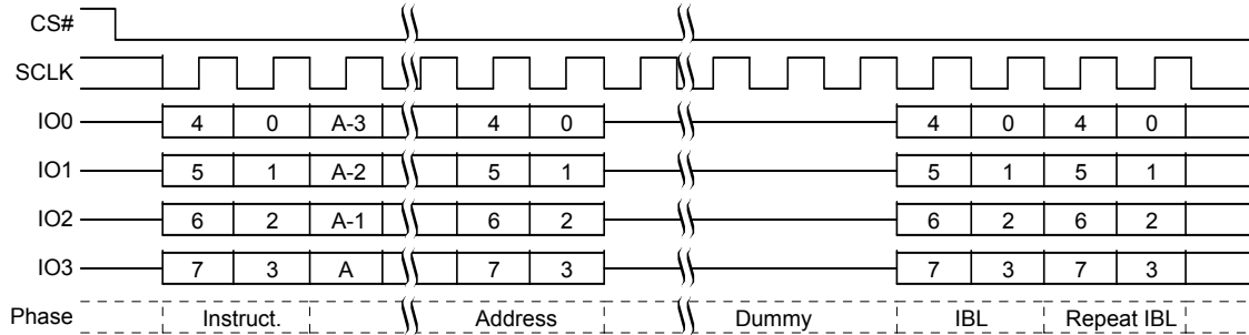
Figure 9.70 IBLRD Command Sequence QPI
