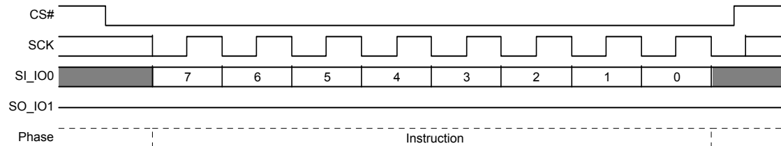
Figure 9.17 Write Disable (WRDI) Command Sequence
