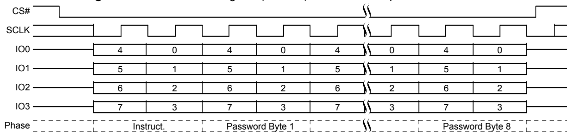
Figure 9.92 Password Program (PASSP) Command Sequence QPI mode
