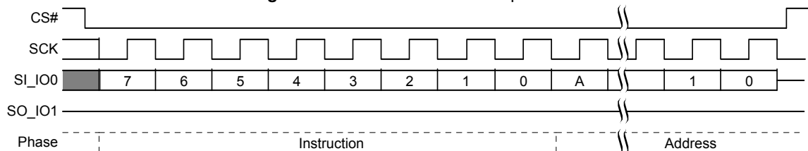
Figure 9.79 SPRP Command Sequence
