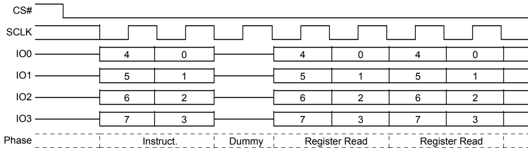
Figure 9.86 Protection Register Read (PRRD) Command Sequence – QPI Mode
