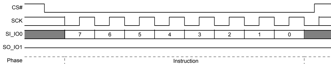
Figure 9.29 Enter 4 Byte Address Mode (4BEN B7h) Command Sequence
