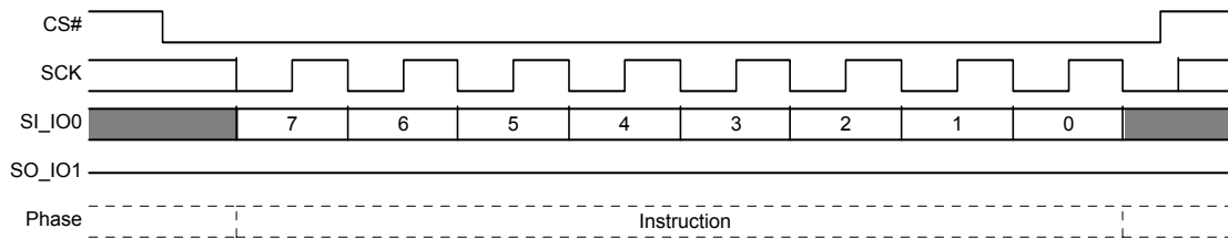
Figure 9.75 Global IBL Lock (GBL) Command Sequence
