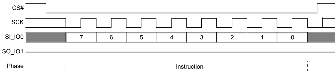
Figure 9.99 Release from Deep Power Down (RES) Command Sequence
