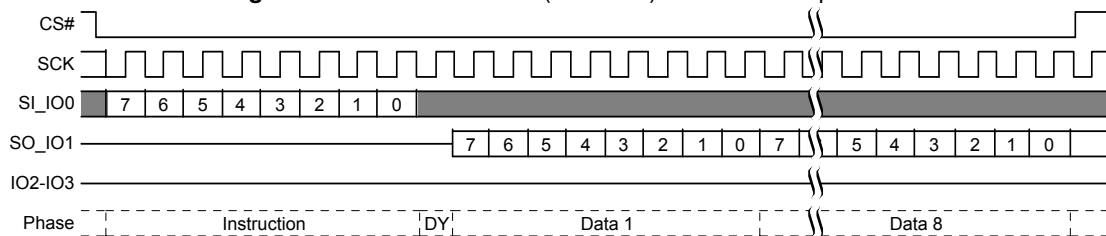
Figure 9.89 Password Read (PASSRD) Command Sequence
