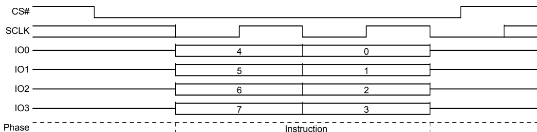
Figure 9.20 Write Enable for Volatile Registers (WRENV) Command Sequence QPI Mode
