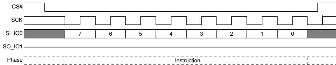
Figure 9.65 Erase or Program Resume command Sequence
