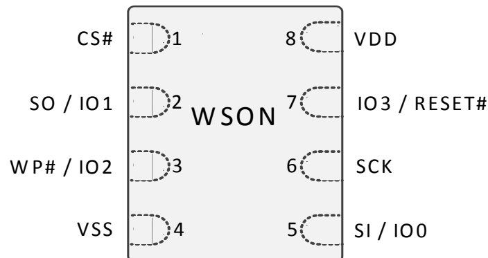
Figure 6.2 8-Connector Package (WSO6 6x8) (WSO6 5x6), Top View
