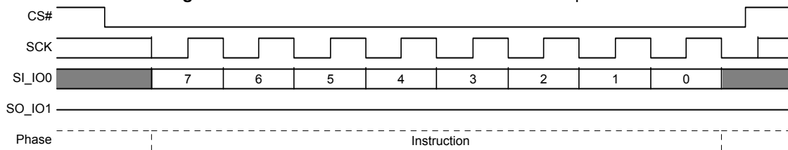
Figure 9.95 Software / Mode Bit Reset Command Sequence
