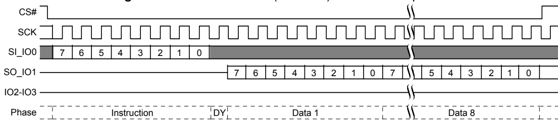
Figure 9.89 Password Read (PASSRD) Command Sequence
