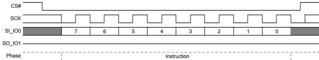
Figure 9.17 Write Disable (WRDI) Command Sequence
