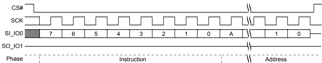
Figure 9.58 Block Erase (BE D8h or 4BE DCh) Command Sequence
