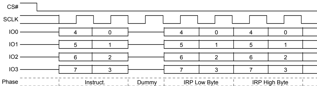
Figure 9.82 IRPRD Command Sequence – QPI Mode
