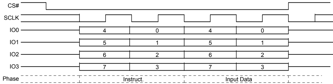
Figure 9.24 Program DLRNV (PDLRNV) Command Sequence – QPI Mode
