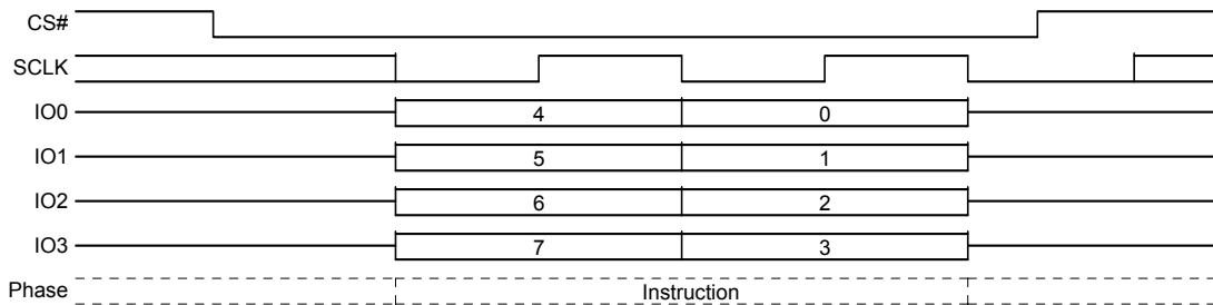
Figure 9.32 Exit 4 Byte Address QPI Mode
