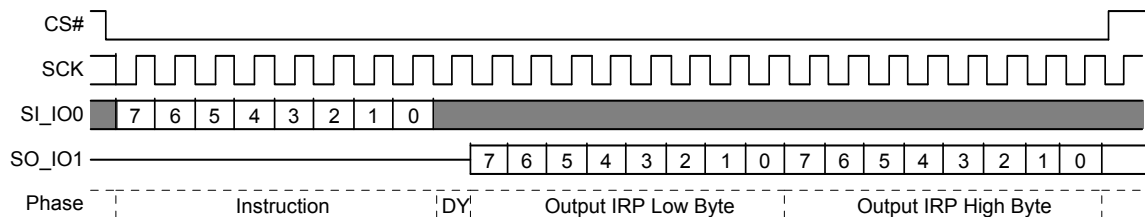
Figure 9.81 IRPRD Command Sequence
