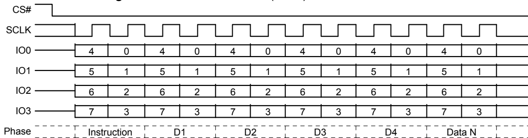
Figure 9.2 Read Identification (RDID) QPI Mode Command
