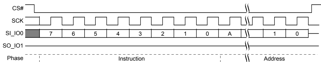
Figure 9.56 Half Block Erase (HBE 52h or 4HBE 53h) Command Sequence
