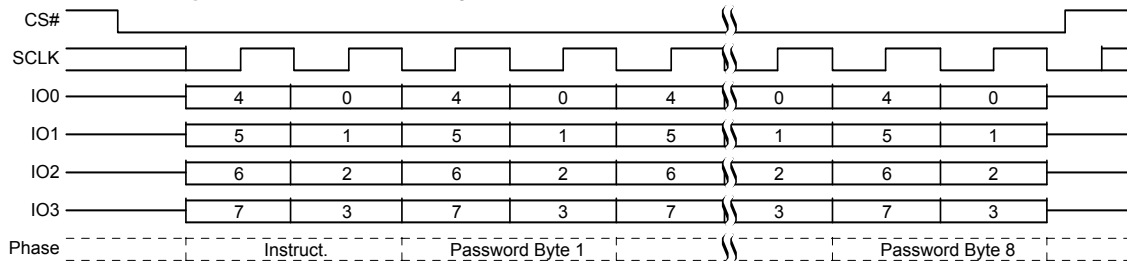
Figure 9.92 Password Program (PASSP) Command Sequence QPI mode
