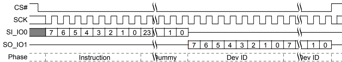
Figure 9.101 Read Identification (RES) Command Sequence
