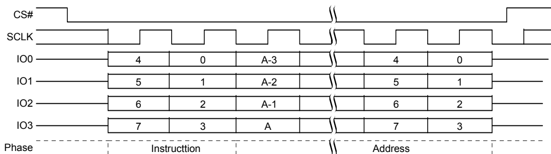
Figure 9.74 IBUL Command Sequence QPI Mode
