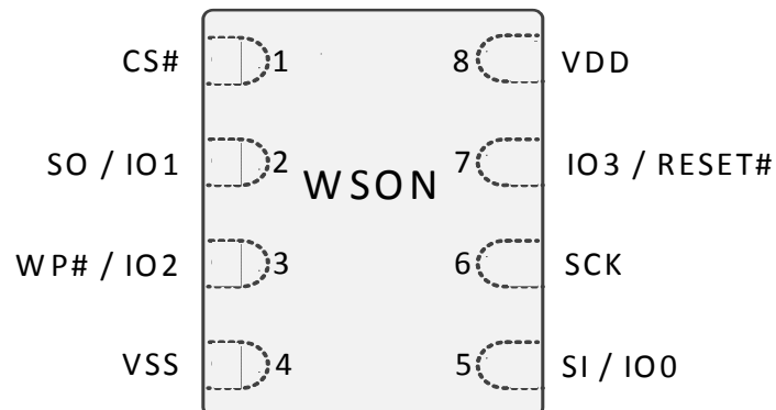
Figure 6.2 8-Connector Package (WSO 6x8) (WSO 5x6), Top View
