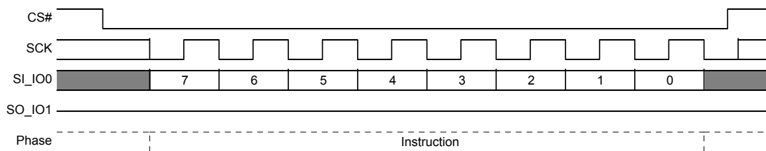
Figure 9.29 Enter 4 Byte Address Mode (4BEN B7h) Command Sequence
