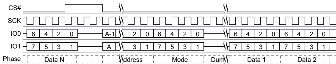
Figure 9.44 Dual I/O Continuous Read Command Sequence
