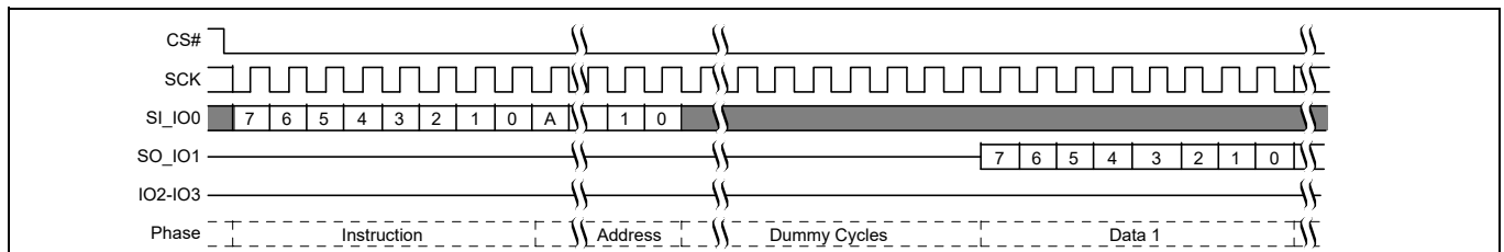
Figure 66 Fast Read (FAST_READ) command sequence [33]
