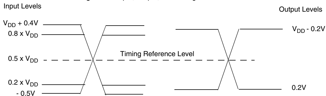
Figure 5.3 Input, Output, and Timing Reference Levels
