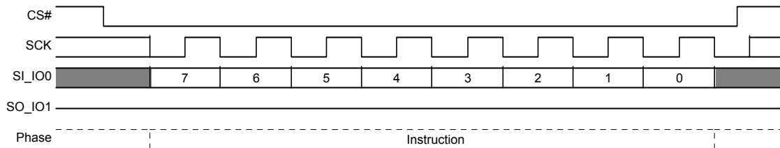
Figure 9.87 Protection Register Lock (PRL) Command Sequence
