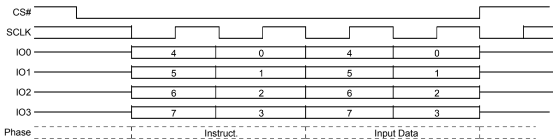
Figure 9.26 Write DLRV (WDLRV) Command Sequence – QPI Mode
