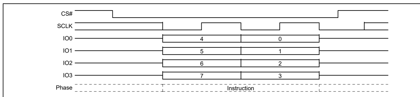
Figure 64 Exit QPI (QPIEX F5h) command sequence
