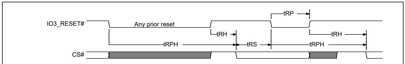
Figure 140 Hardware reset when Quad or QPI mode is not enabled and IO3 / RESETE# is enabled
