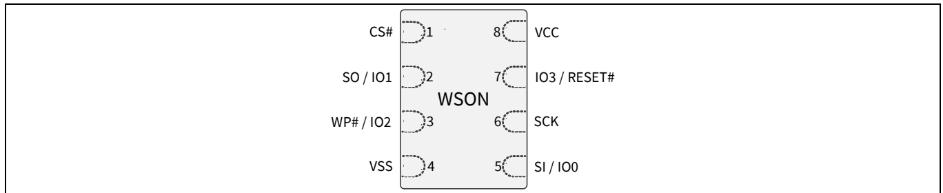
Figure 4 8-connector package (WSO5N 5 x 6), top view [2]
