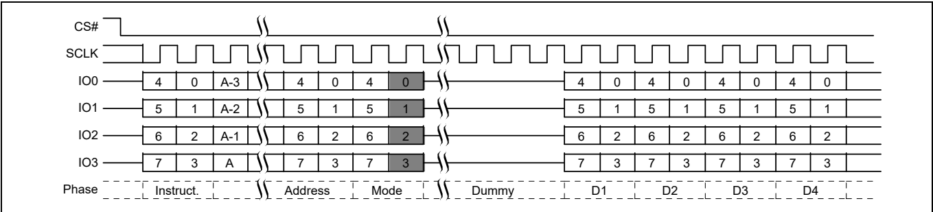
Figure 72 Quad I/O Read initial access command sequence QPI mode [38]
