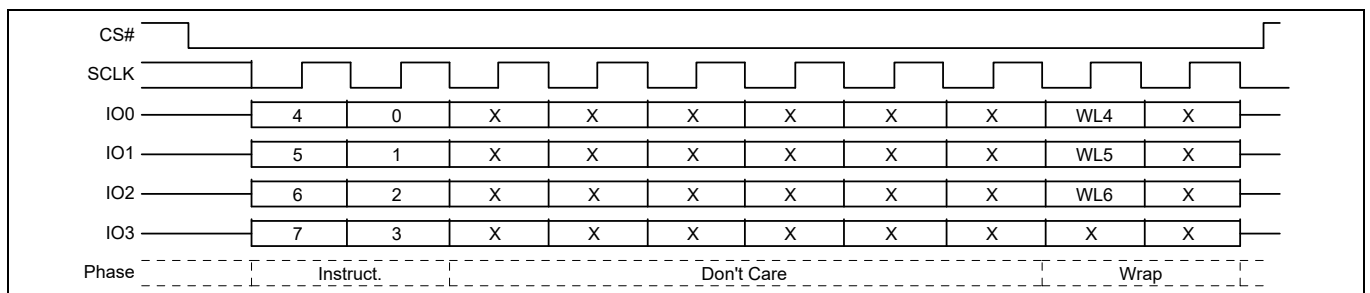
Figure 62 Set Burst Length command sequence QPI mode
