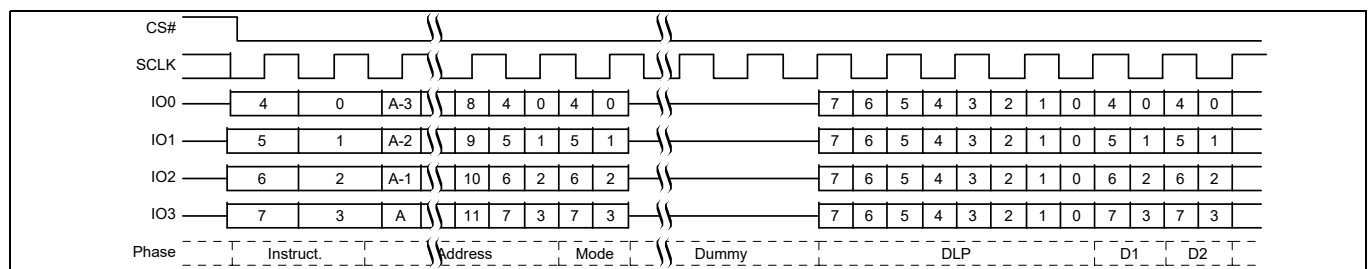
Figure 75 DDR Quad I/O Read initial access QPI mode [40, 42]
