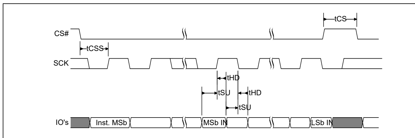
Figure 147 SPI DDR input timing
