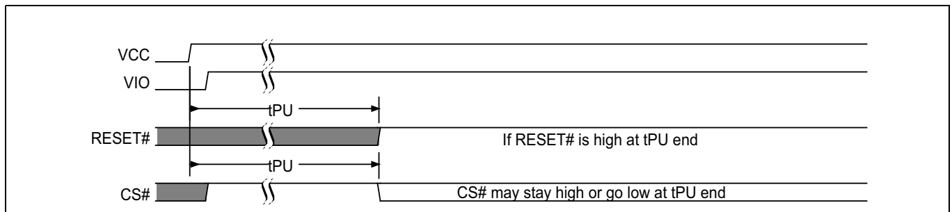
Figure 27 Reset HIGH at the end of POR
