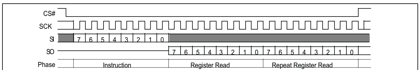
Figure 53 Read configuration register (RDCR 35h) command sequence
