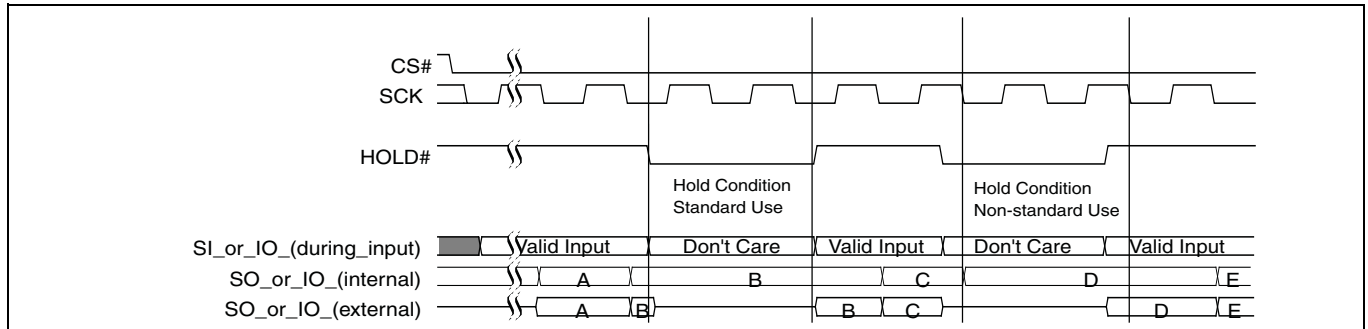
Figure 1 HOLD mode operation
