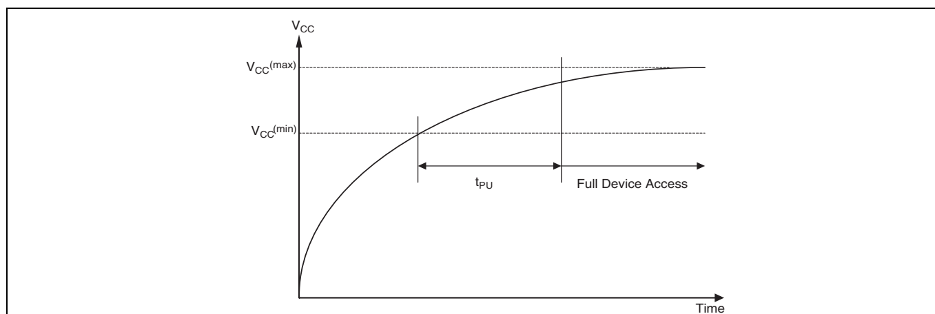
Figure 21 Power-up
