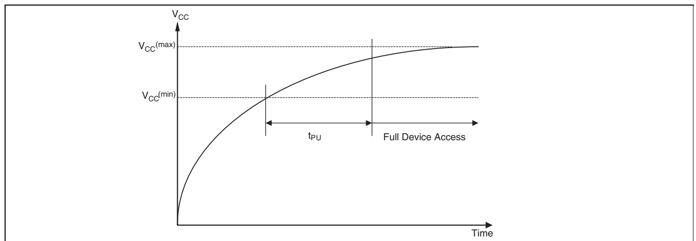
Figure 25 Power-up
