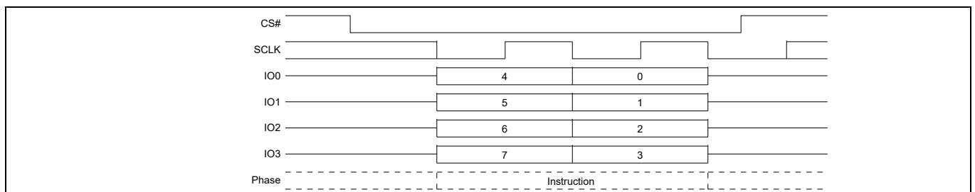
Figure 49 Write Enable (WREN) command sequence QPI mode
