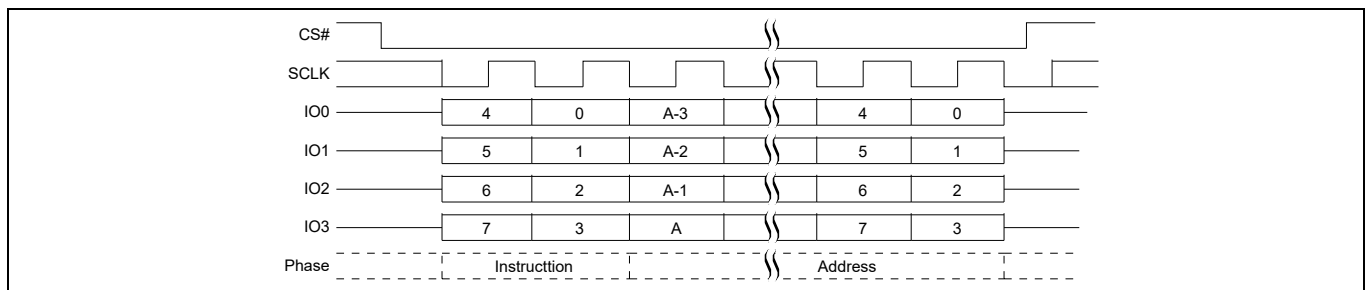
Figure 84 EES QPI mode command sequence [56]
