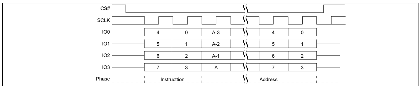
Figure 78 Parameter Sector Erase (P4E 20h or 4P4E 21h) QPI mode command sequence [53]
