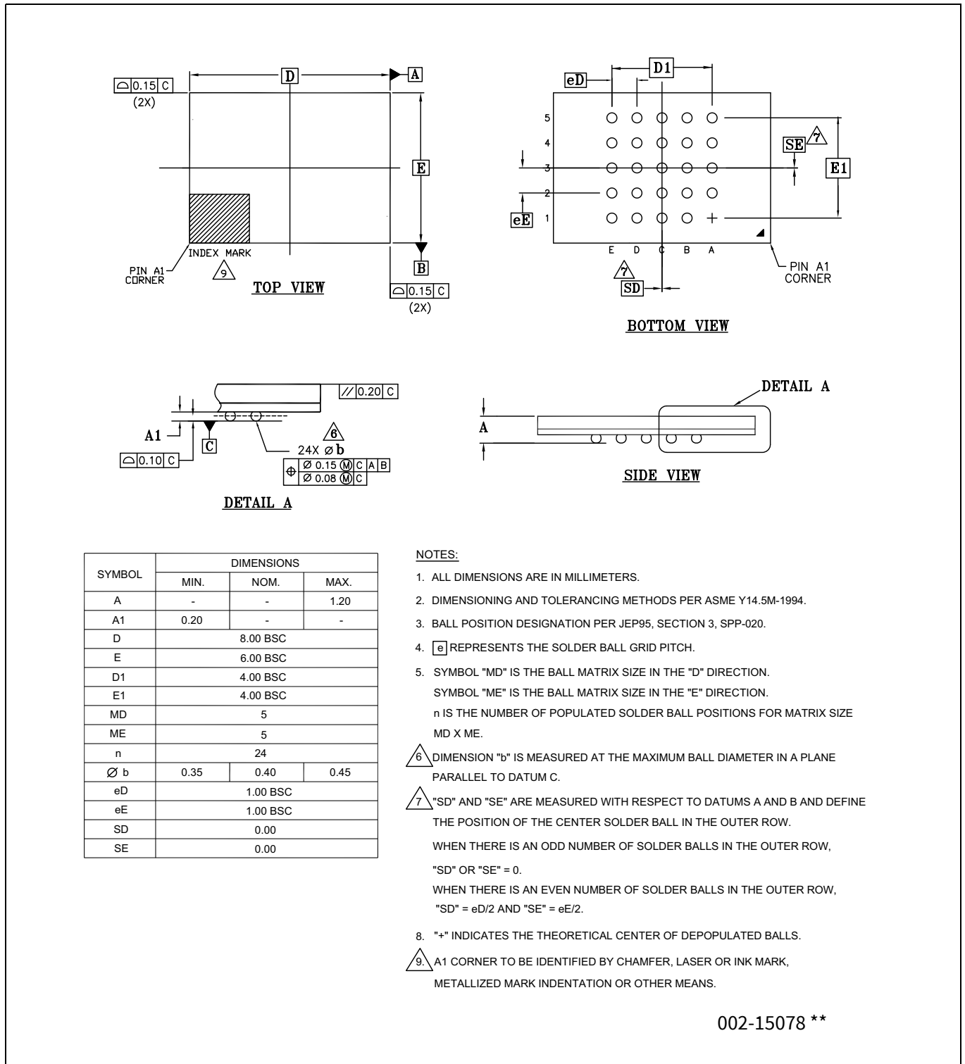
Figure 39 Package outline, 24-Ball FBGA 8.0 x 6.0 x 1.2 MM ZSA024
