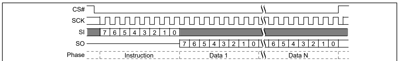
Figure 43 Read Identification (RDID) command sequence
