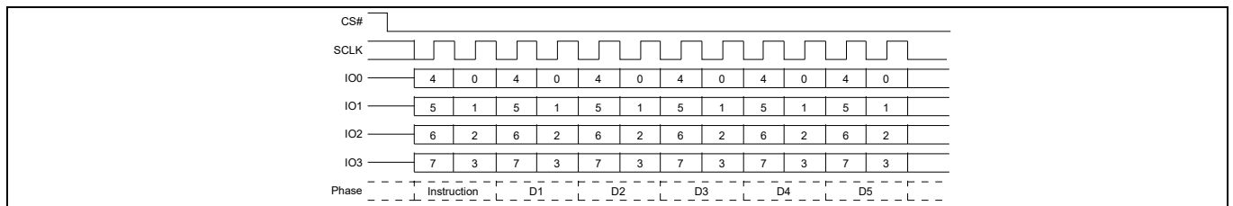
Figure 45 Read Quad Identification (RDQID) command sequence
