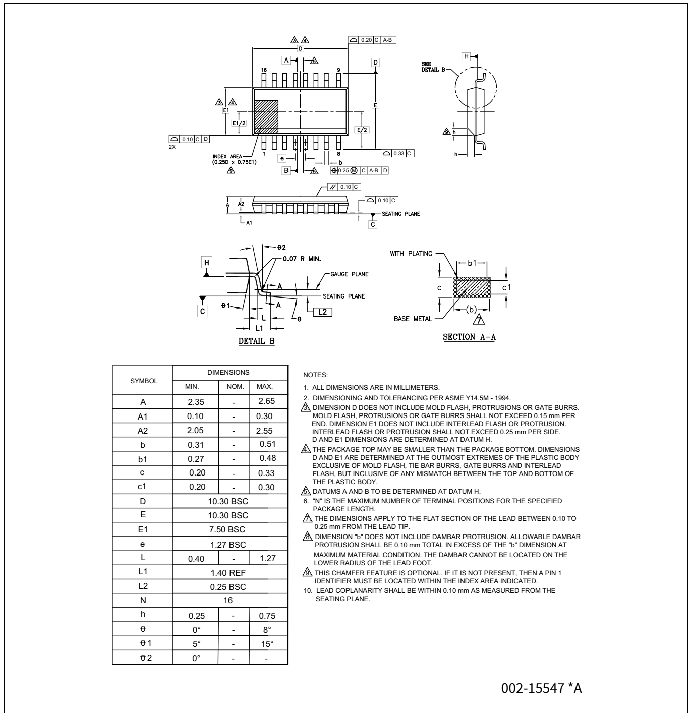
Figure 38 Package outline, 16 LEAD SOIC 10.30 x 7.50 x 2.65 SL3016 (PG-DSO-16-806)
