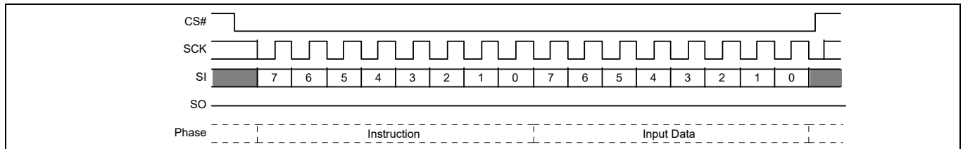
Figure 57 Write VDLR (WVDLR) command sequence
