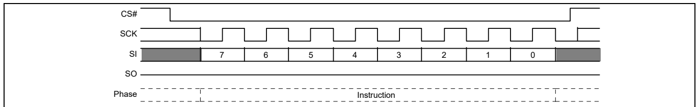
Figure 104 Mode Bit Reset command sequence
