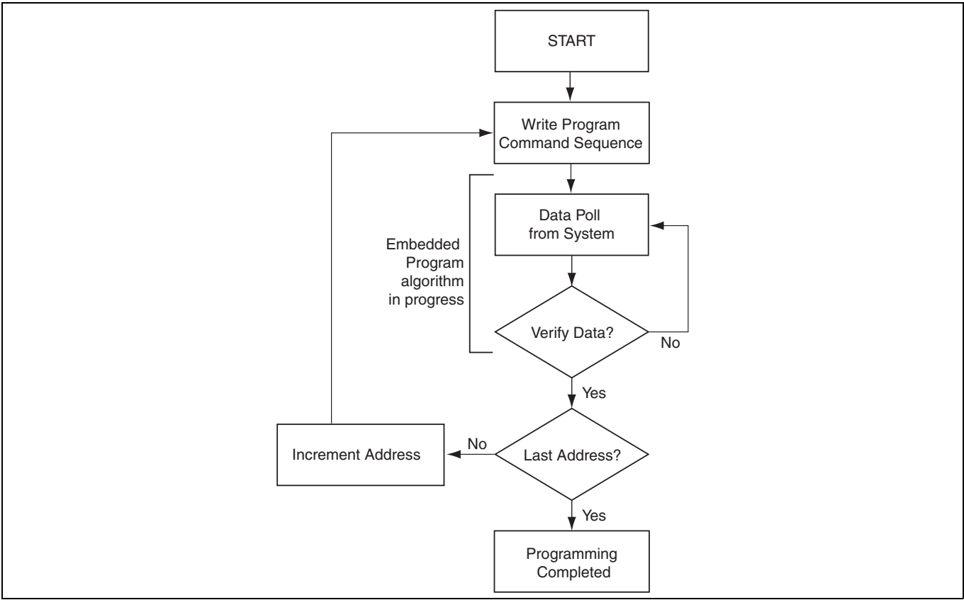
Figure 10 Program operation
