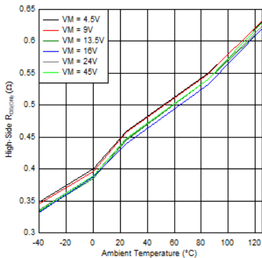
Figure 6-9. High-Side R_{DS(ON)} over Temperature
