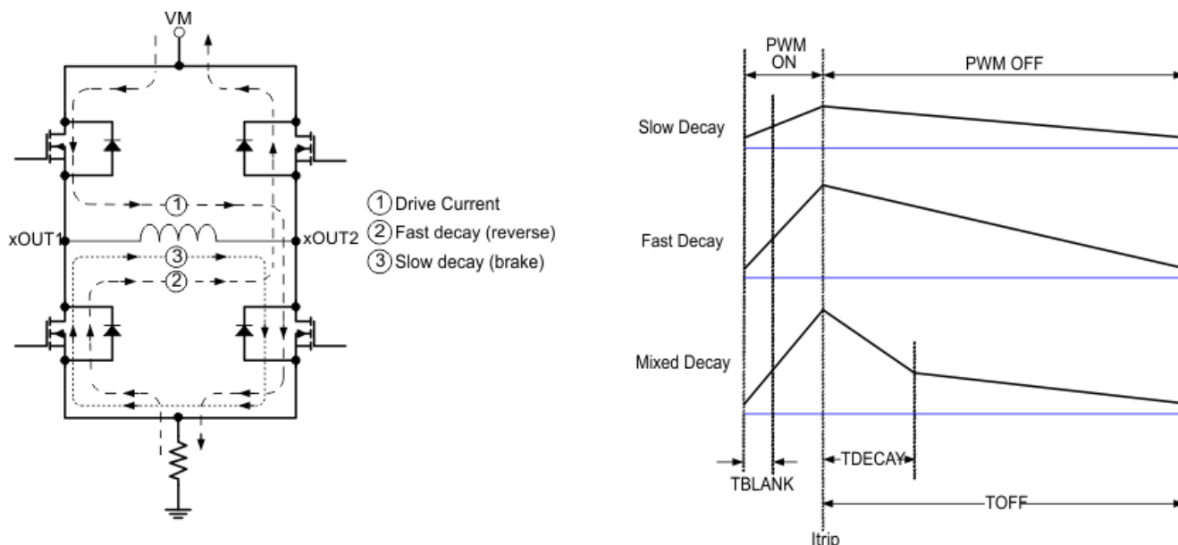
Figure 7-7. Decay Modes
