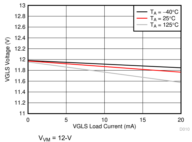
Figure 7-10. VGLS Voltage Over Load Current
