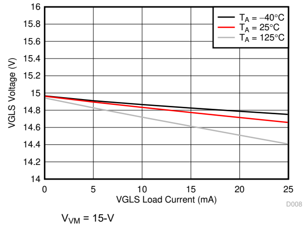
Figure 7-8. VGLS Voltage Over Load Current
