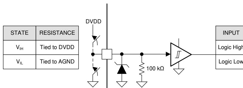
Figure 8-20. Logic-Level Input Pin Structure
