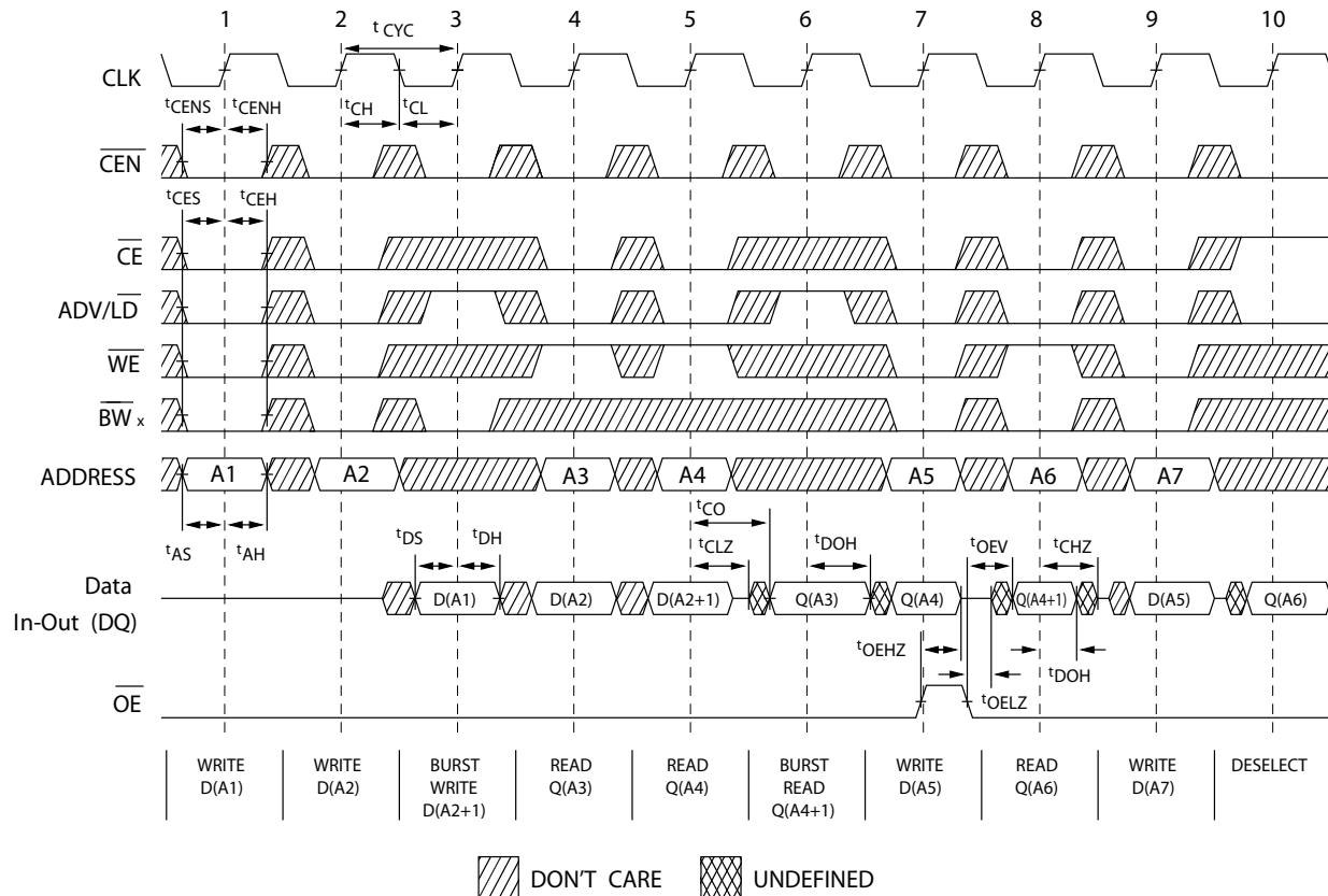
Figure 5. Read/Write Timing [27, 28, 29]
