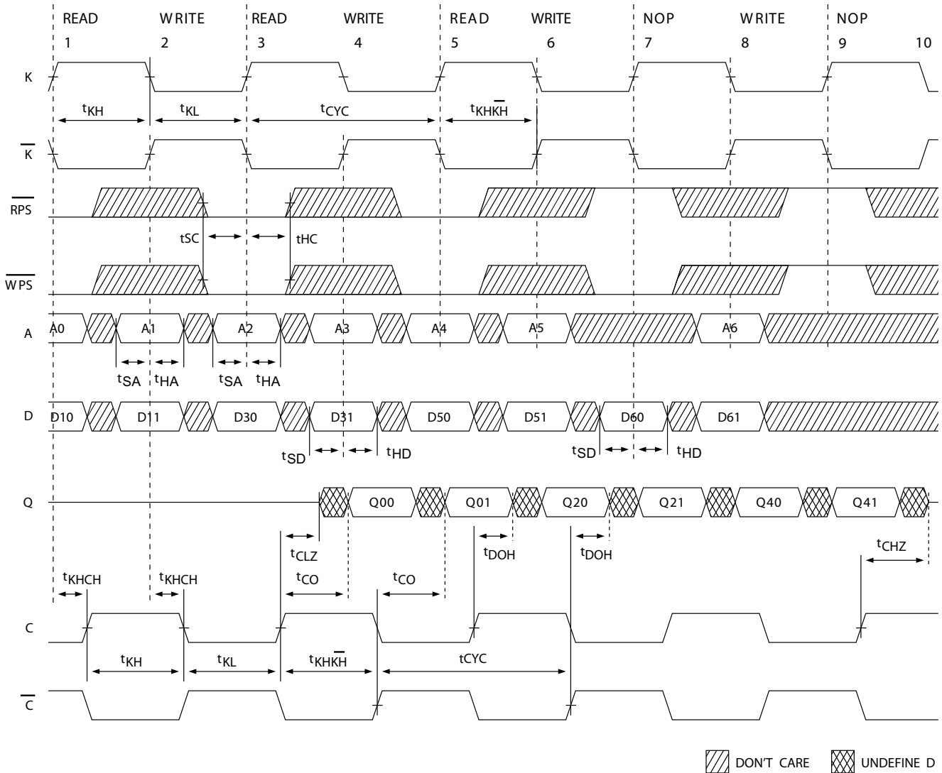
Figure 5. Switching Waveforms [29, 30, 31]
