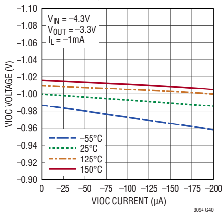
VIOC Voltage
