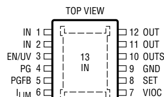
MSE PACKAGE 12-LEAD PLASTIC MSOP T_{JMAX} = 150^{\circ}\text{C} , \theta_{JA} = 33^{\circ}\text{C/W} , \theta_{JC} = 8^{\circ}\text{C/W} EXPOSED PAD (PIN 13) IS IN, MUST BE SOLDERED TO PCB
