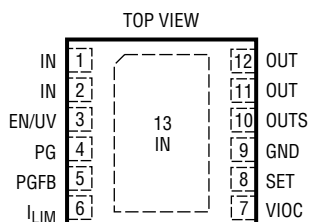
DD PACKAGE 12-LEAD (3mm × 3mm) PLASTIC DFN T_{JMAX} = 150^{\circ}\text{C} , \theta_{JA} = 34^{\circ}\text{C/W} , \theta_{JC} = 5.5^{\circ}\text{C/W} EXPOSED PAD (PIN 13) IS IN, MUST BE SOLDERED TO PCB
