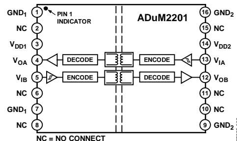
Figure 2. ADuM2201
