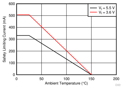
Figure 8-1. Thermal Derating Curve for Limiting Current per VDE
