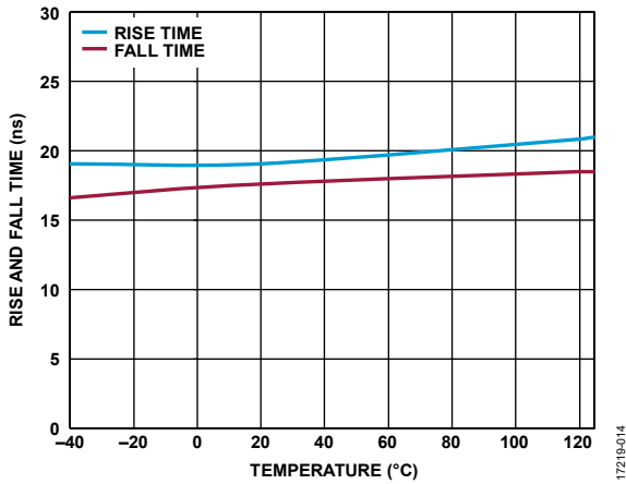
Figure 21. Rise and Fall Time vs. Temperature with a 3.9\Omega Series Gate Resistor for a 2\text{ nF} Load and a 15\text{ V} Output Supply
