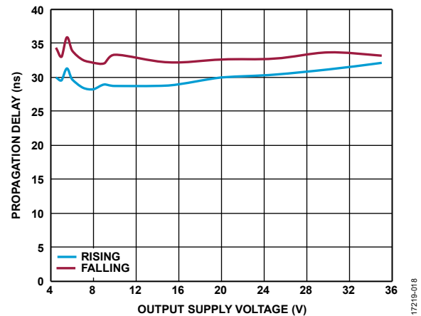
Figure 25. Propagation Delay vs. Output Supply Voltage, Rising and Falling, V_{DD1} = 5\text{ V}
