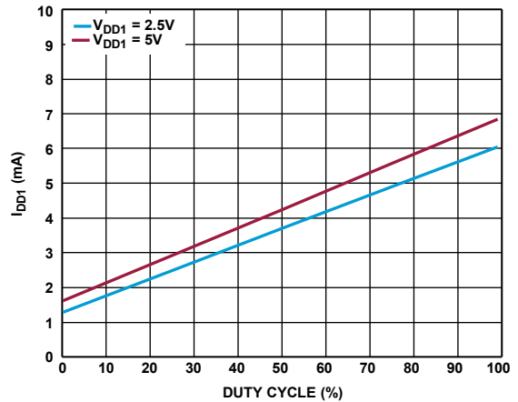
Figure 19. I_{DD1} vs. Duty Cycle for V_{DD1} = 2.5\text{ V} and V_{DD1} = 5\text{ V} , V_{DD2} = 15\text{ V} ( V_{DD2} Refers to V_{DDA} or V_{DDB} )
