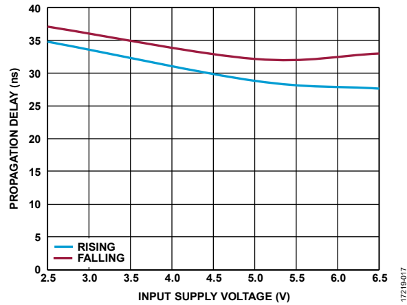
Figure 24. Propagation Delay vs. Input Supply Voltage, Rising and Falling, V_{DD2} = 15\text{ V} ( V_{DD2} Refers to V_{DDA} or V_{ddb} )
