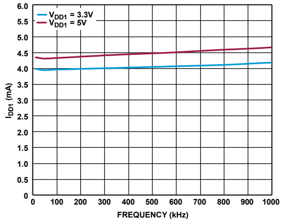
Figure 17. V_{DD1} Current ( I_{DD1} ) vs. Frequency for V_{DD1} = 3.3\text{ V} and V_{DD1} = 5\text{ V} , 50% Duty Cycle
