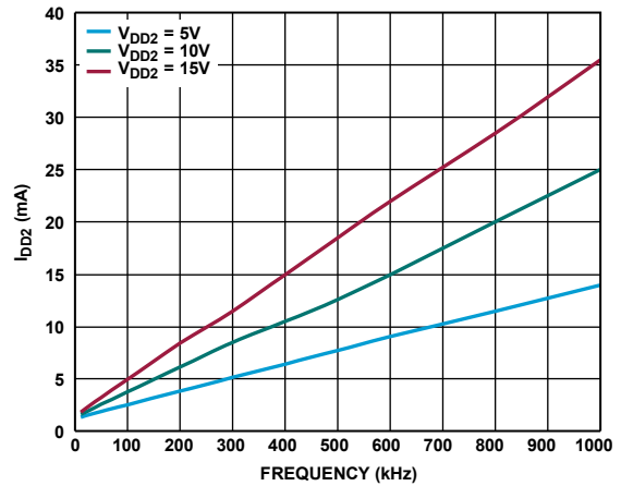
Figure 18. V_{DD2} Current ( I_{DD2} ) vs. Frequency for V_{DD2} = 5\text{ V} , V_{DD2} = 10\text{ V} , and V_{DD2} = 15\text{ V} , 50% Duty Cycle, 2 nF Load ( V_{DD2} Refers to V_{DDA} or V_{DDB} )
