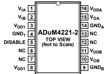
Figure 7. ADuM4221-2 Pin Configuration
