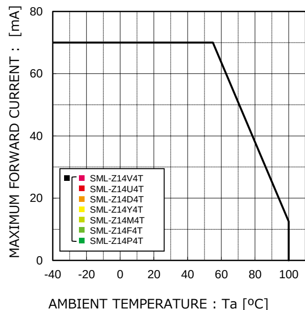
Fig.4 Derating
