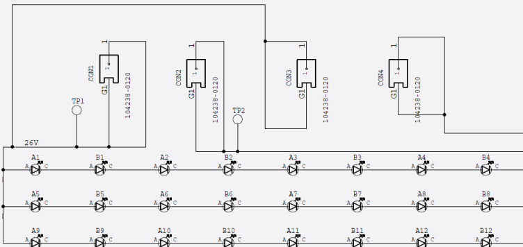
M282C_G2 (8S3P)
