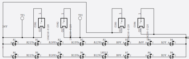
M282B_G2 (8S2P)
